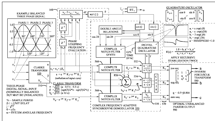
COMPLEX NOTCH FILTER APPROACH
