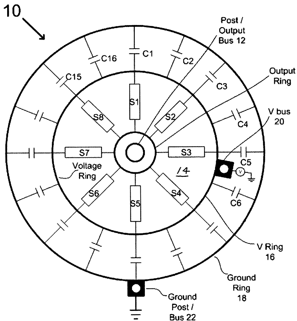
Basic Ring Network
