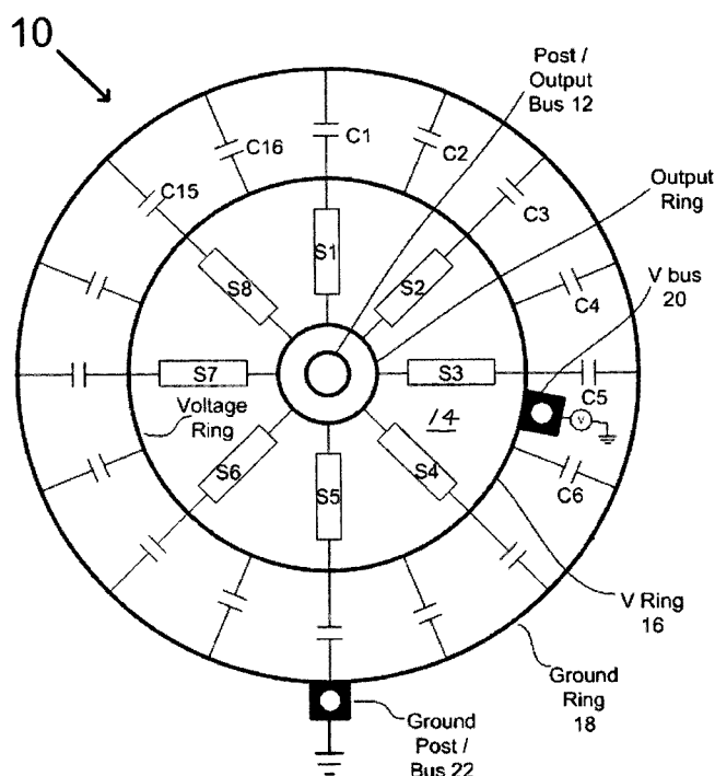
Basic Ring Network
