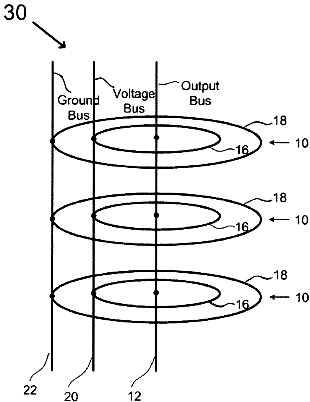
Stacked Switch Ring Network
