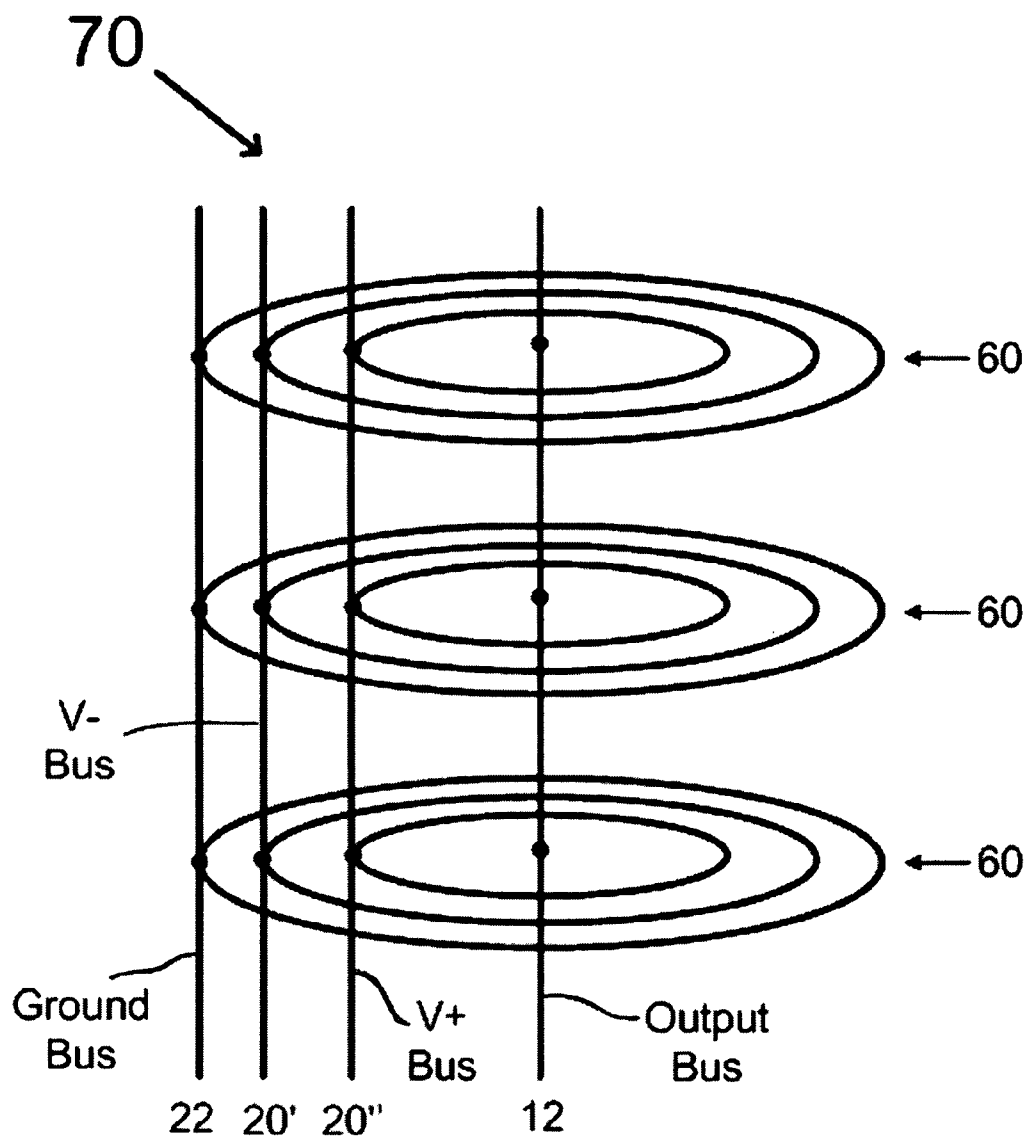
Stacked Half Bridge Ring Networks
