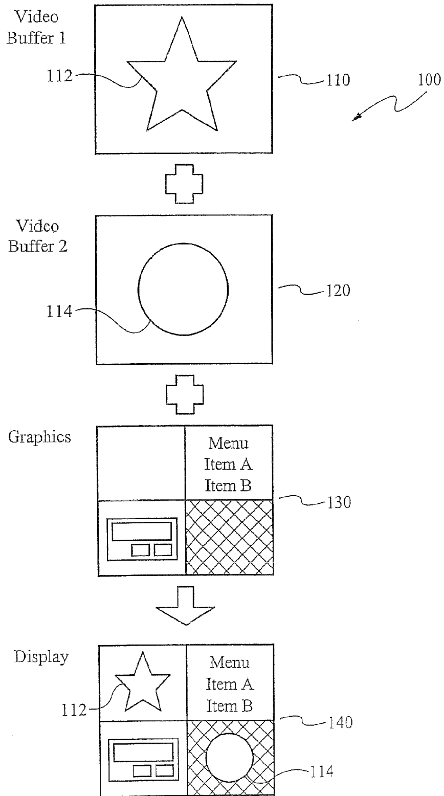
Fig. 1 (PRIOR ART)
