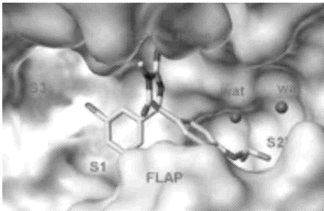
Compound 1A
