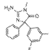
Compound 1B
