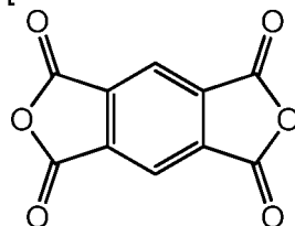
[Chemical Formula A15]
