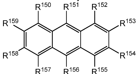
[Chemical Formula 15]
