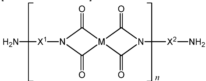
[Chemical Formula 9]
