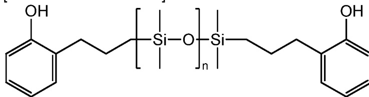
[Chemical Formula A8]
