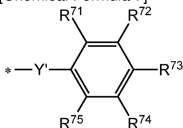
[Chemical Formula 7]
