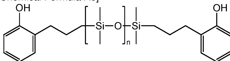
[Chemical Formula A6]
