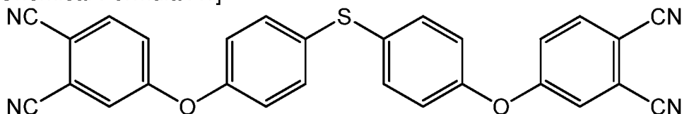
[Chemical Formula A1]
