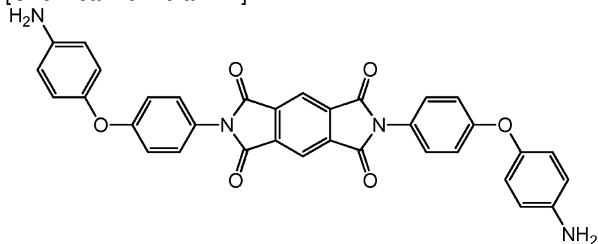
[Chemical Formula A14]
