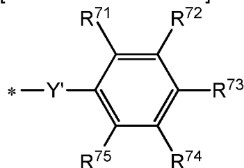
[Chemical Formula 7]
