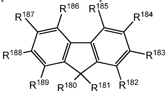
[Chemical Formula 18]
