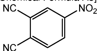
[Chemical Formula A3]
