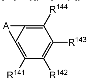
[Chemical Formula 14]
