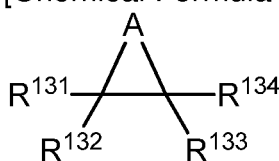
[Chemical Formula 13]
