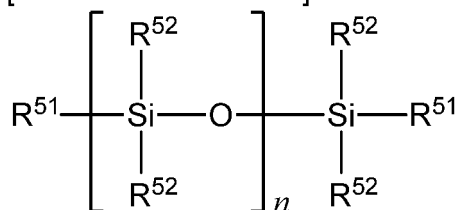
[Chemical Formula 8]
