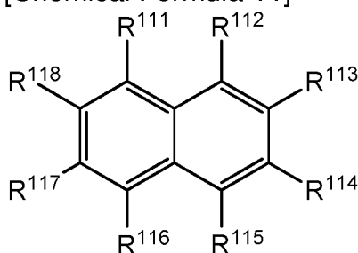
[Chemical Formula 11]
