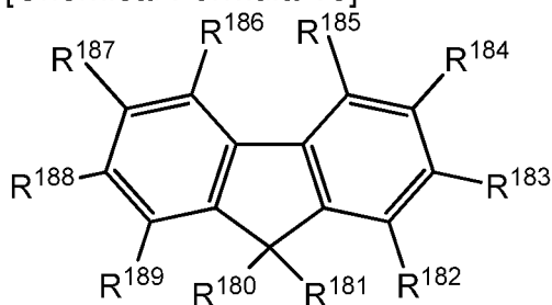
[Chemical Formula 18]
