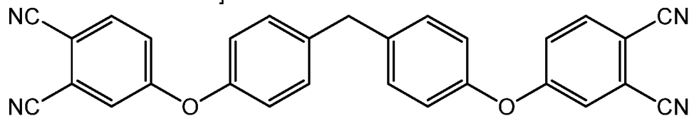
[Chemical Formula A4]
