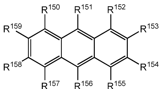
[Chemical Formula 15]
