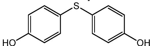
[Chemical Formula A2]
