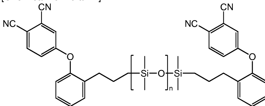
[Chemical Formula A7]
