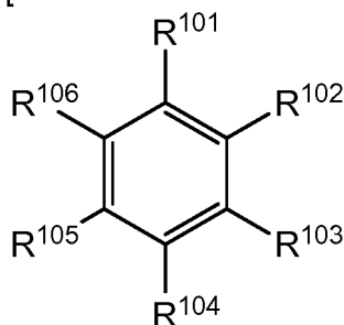
[Chemical Formula 10]
