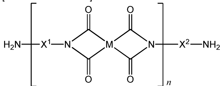
[Chemical Formula 9]
