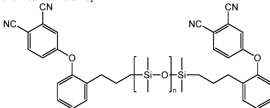
[Chemical Formula A5]
