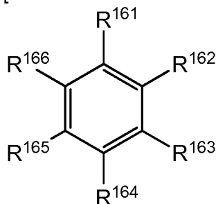
[Chemical Formula 16]
