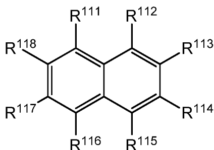
[Chemical Formula 11]
