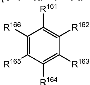
[Chemical Formula 16]
