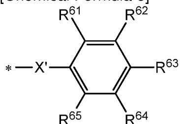
[Chemical Formula 6]
