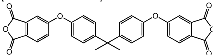
[Chemical Formula A17]
