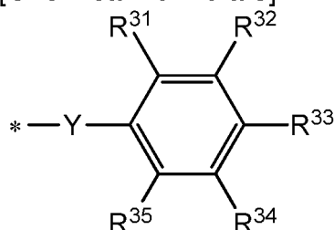
[Chemical Formula 3]
