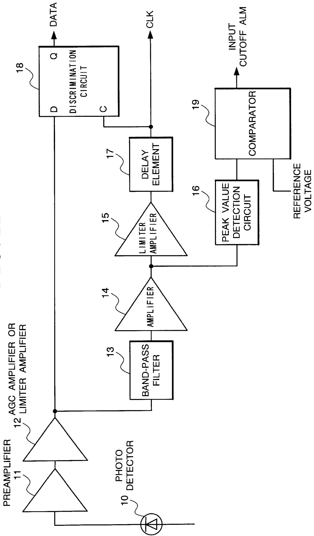
FIG. 12 (PRIOR ART)
