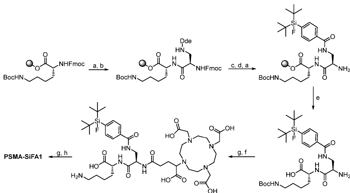
Scheme 1: Synthesis of PSMA-SiFA1: a) 20% piperidine (DMF); b) Fmoc-D-Dap(Dde)-OH, HOBt, TBTU, DIPEA (DMF); c) imidazole, hydroxylamine hydrochloride, (NMP, DMF); d) SIFA-BA, HOBt, TBTU, DIPEA (DMF); e) TFE, AcOH, (DCM); f) DOTAGA-anhydride, DIPEA, (DMF); g) TFA; h) PfpO-Sub-(tBuO)KuE(OtBu) 2 , TEA, (DMF).
