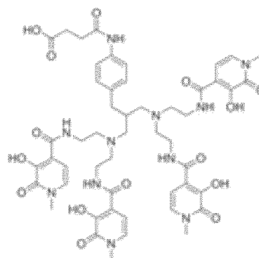
Me-3,2-HOPO
