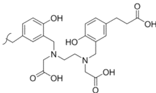
HBED
