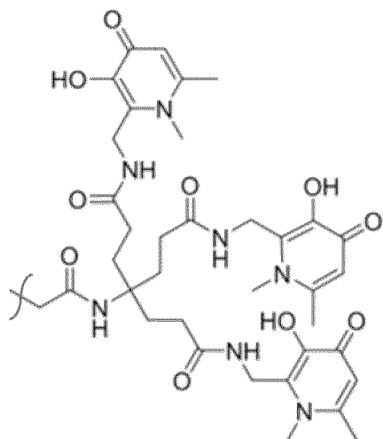
THP
