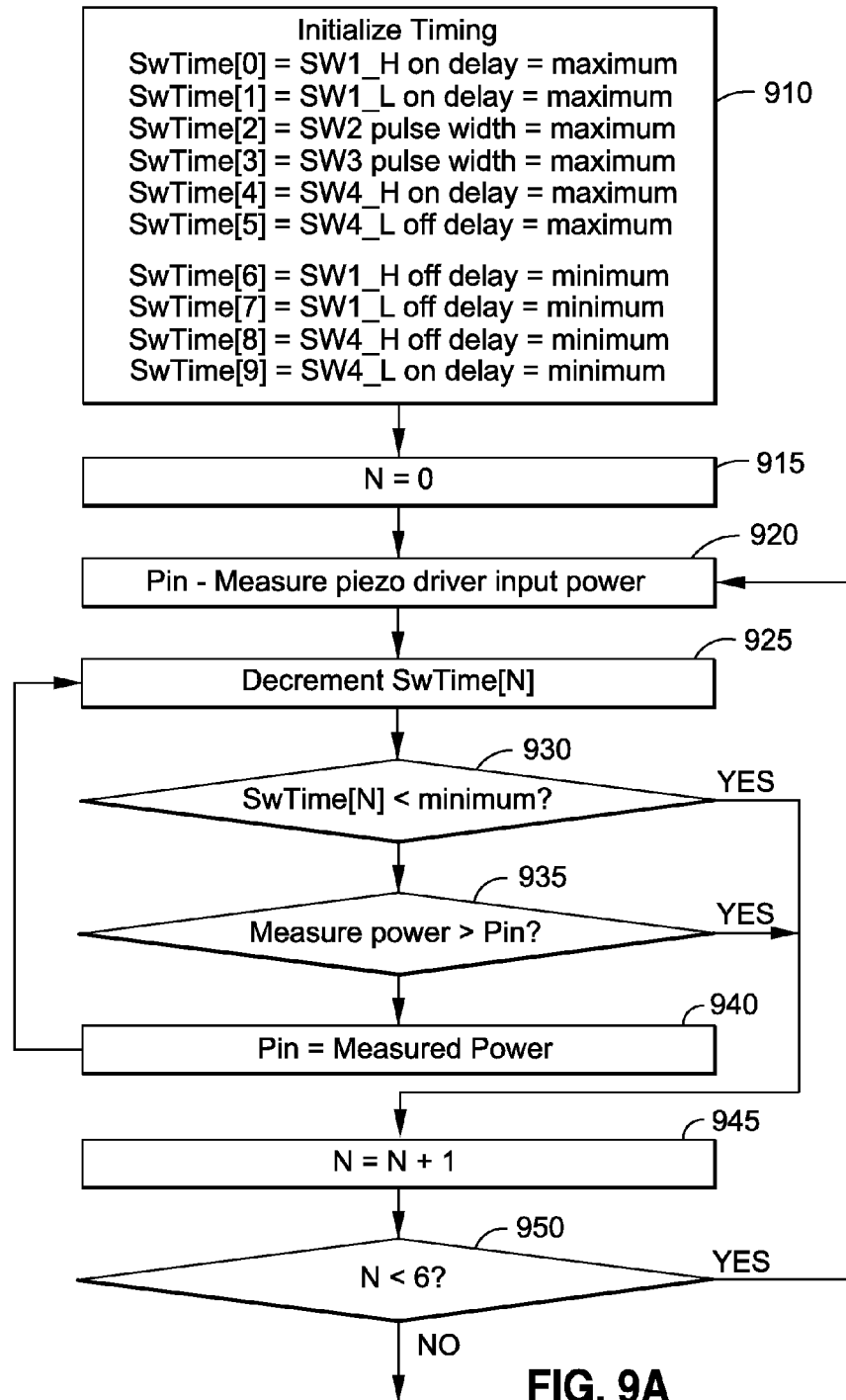
Exemplary Piezo Power Optimization Algorithm Flow Chart
