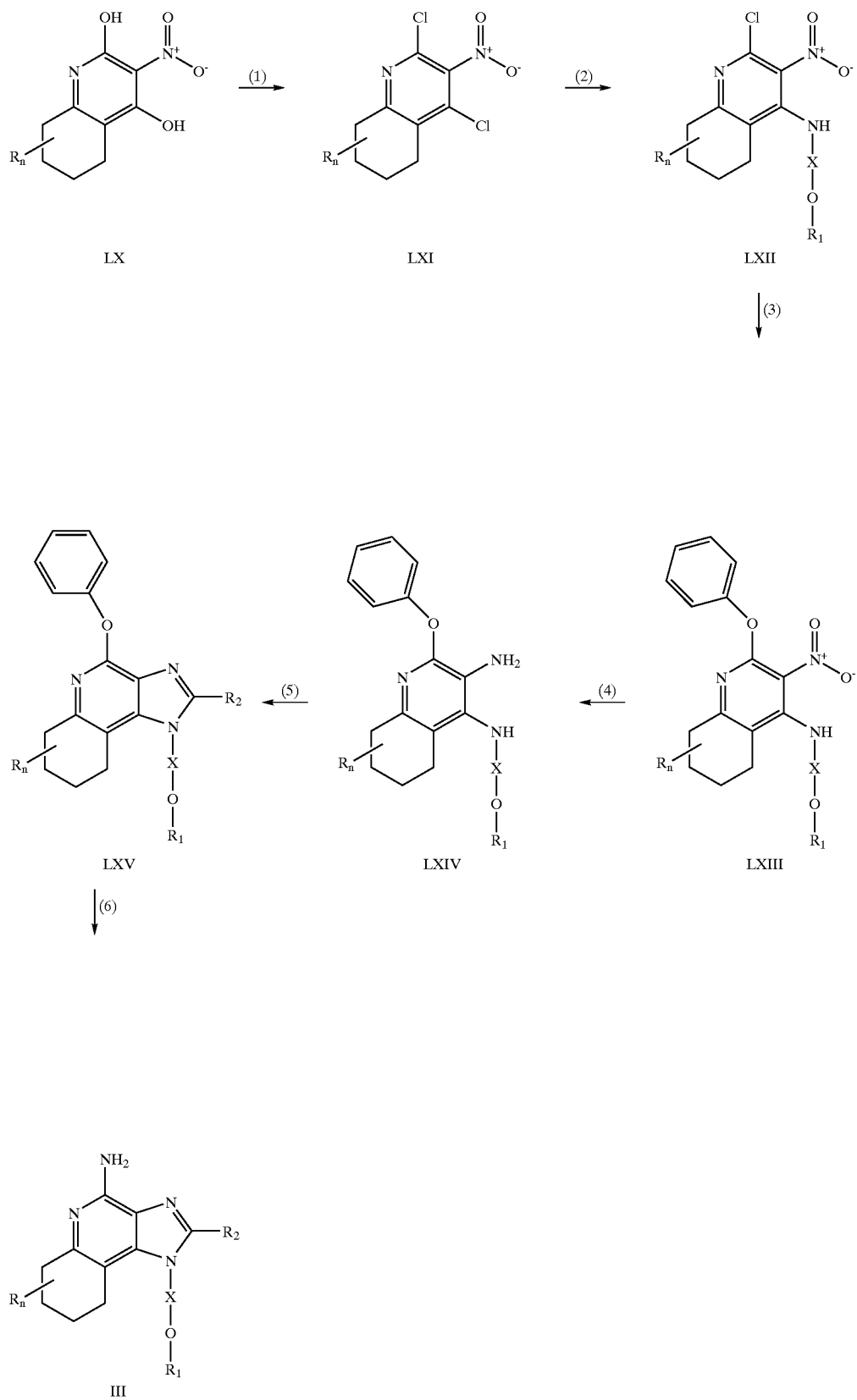
Reaction Scheme XVI
