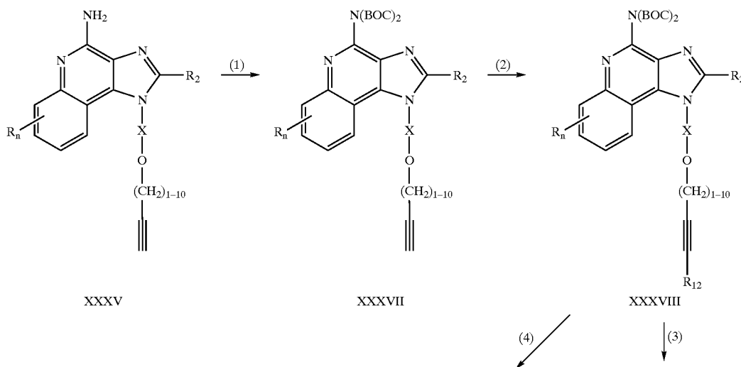
Reaction Scheme VIII
