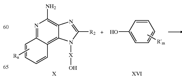
Reaction Scheme III
