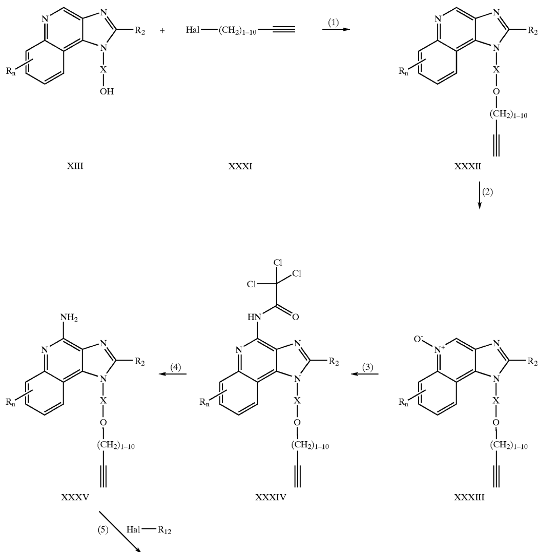
Reaction Scheme VII
