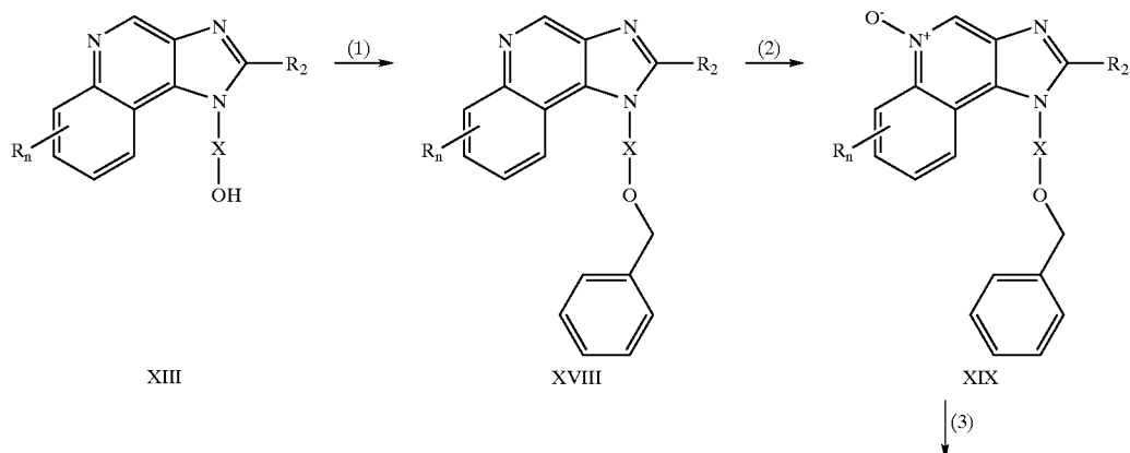
Reaction Scheme IV
