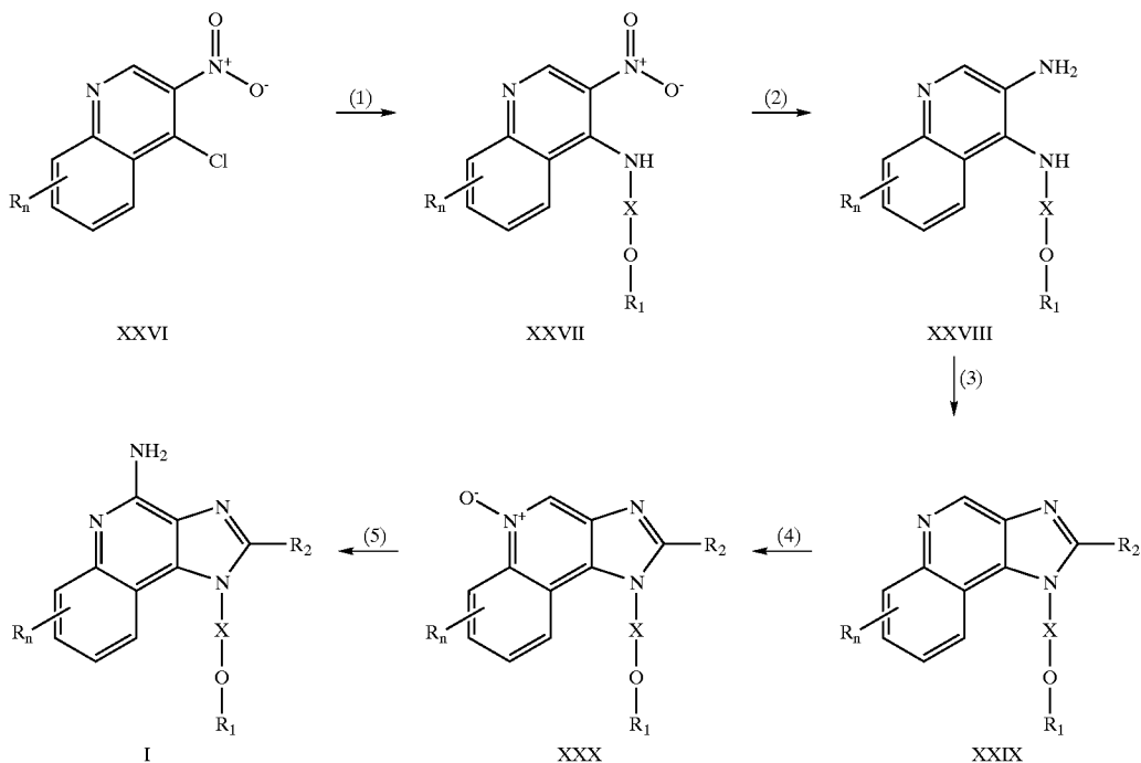
Reaction Scheme VI
