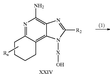
Reaction Scheme XV
