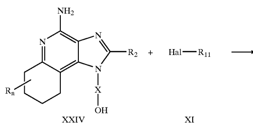
Reaction Scheme V
