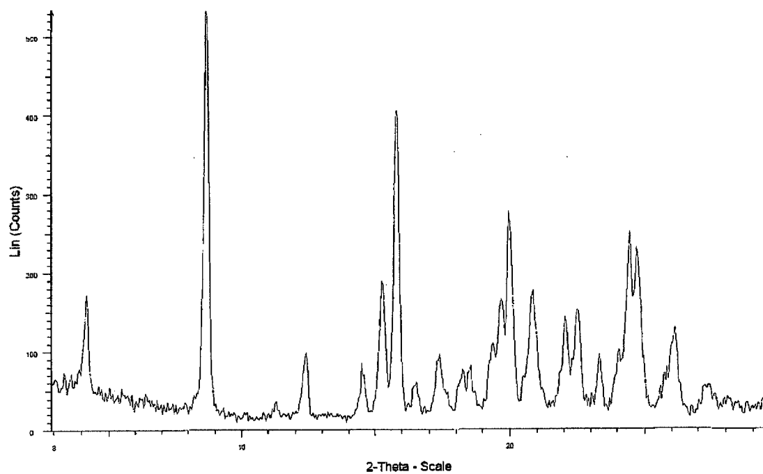
Figure 10 XRPD of Form II
