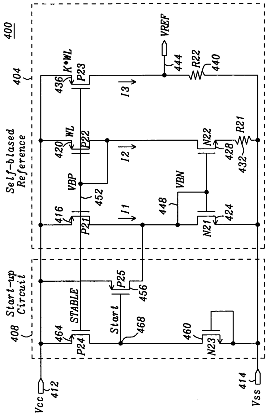
FIG. 5 - Prior Art
