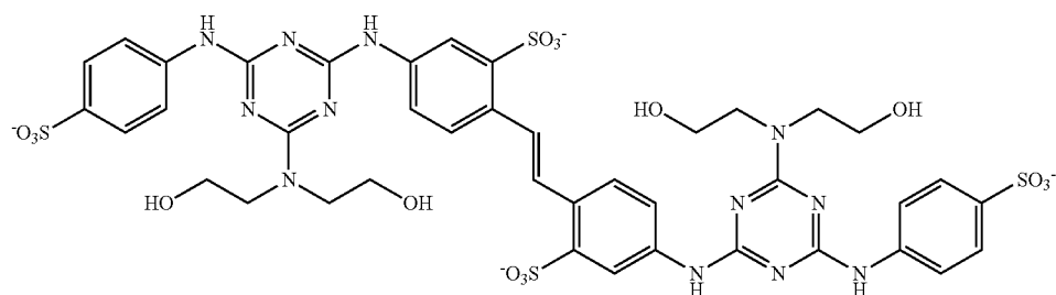
Tinopal DCS (Ciba)
