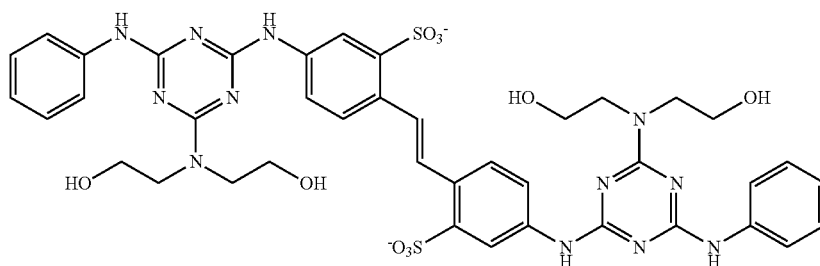
Tinopal UNPA-GX (Ciba)
