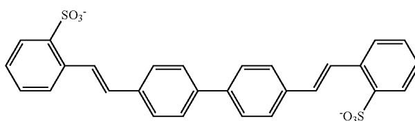
Tinopal CBS—X (Ciba) Disodium 4,4'-bis-(2-sulfostyryl)biphenyl
