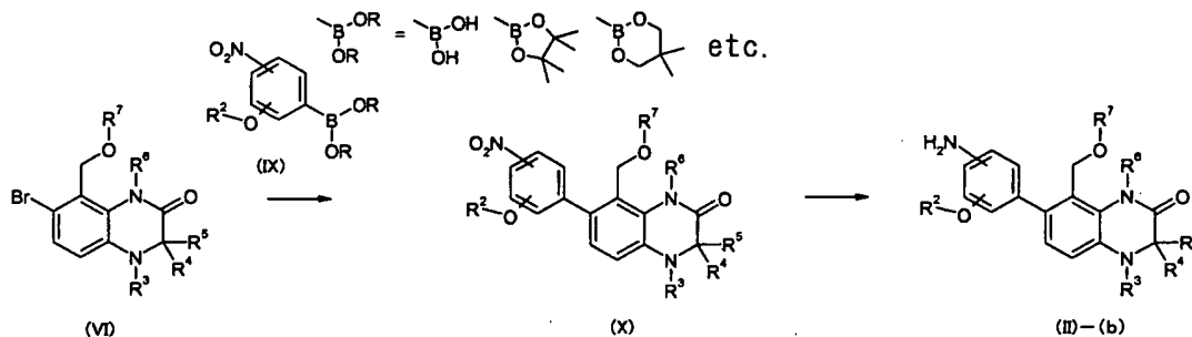
Synthetic Route 4
