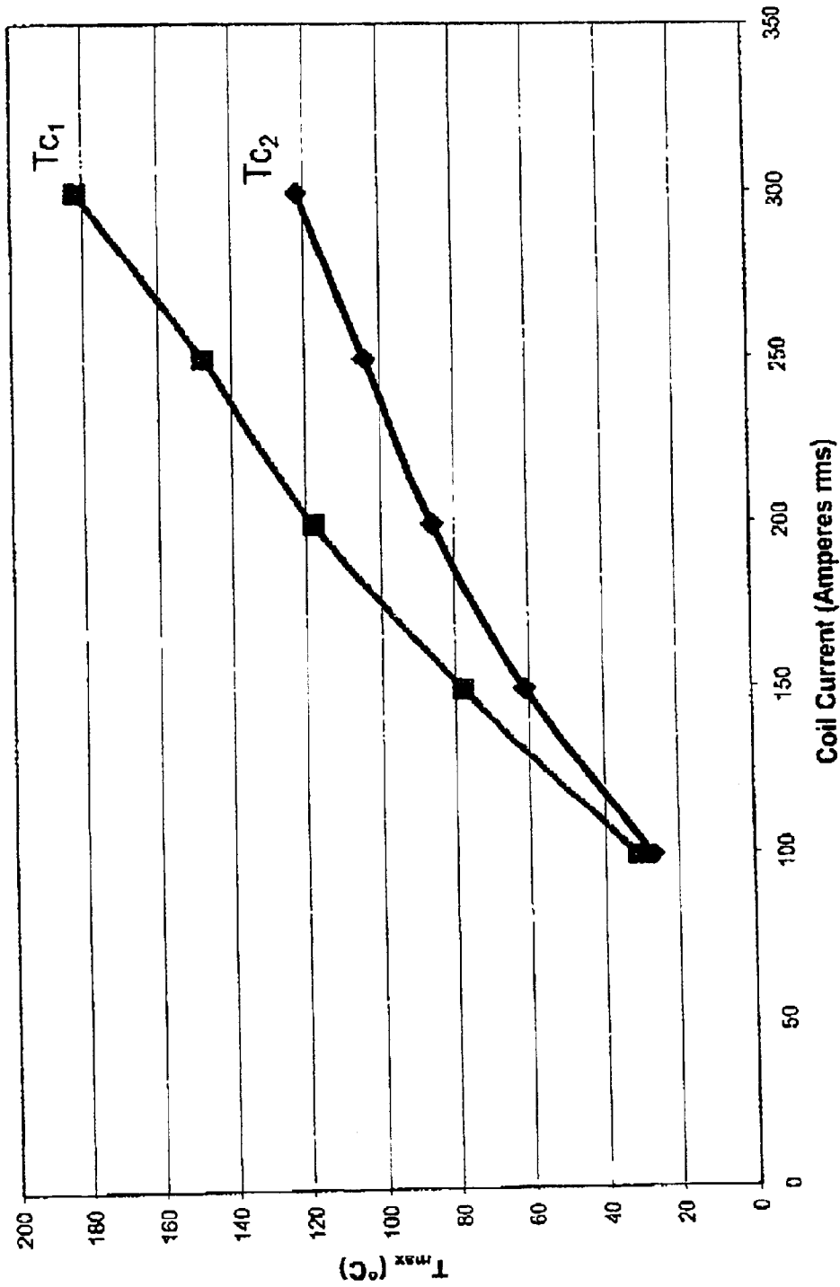
FIG. 7 EFFECT OF FERROFLUID CURIE POINT ON WINDING TEMPERATURE AT VARYING CURRENTS
