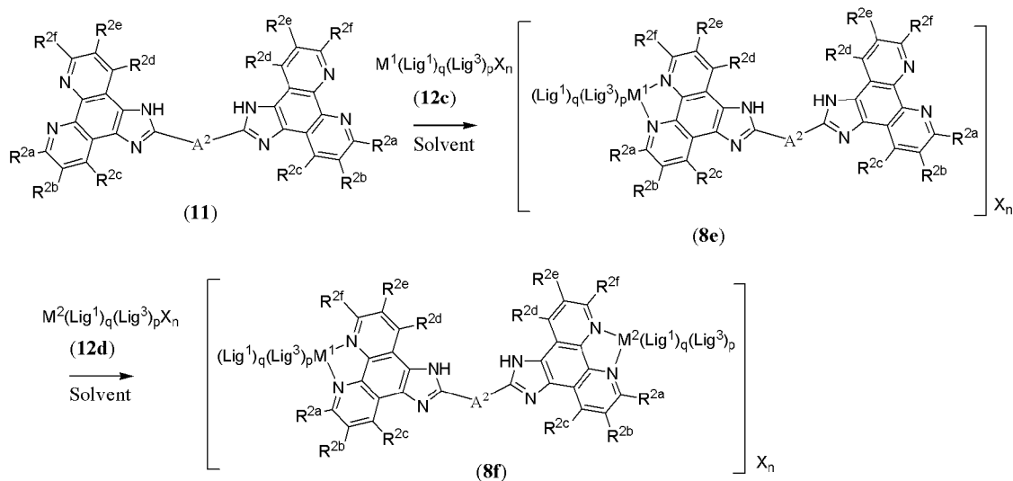
Scheme 3d
