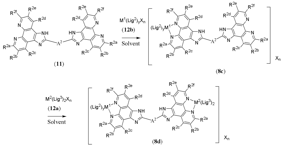
Scheme 3c
