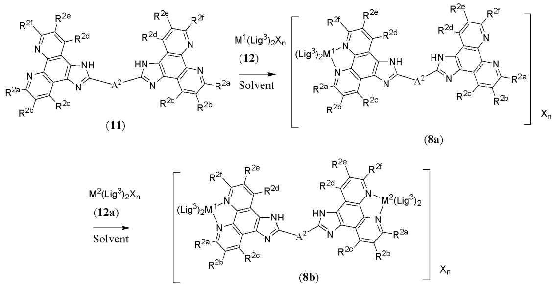
Scheme 3b
