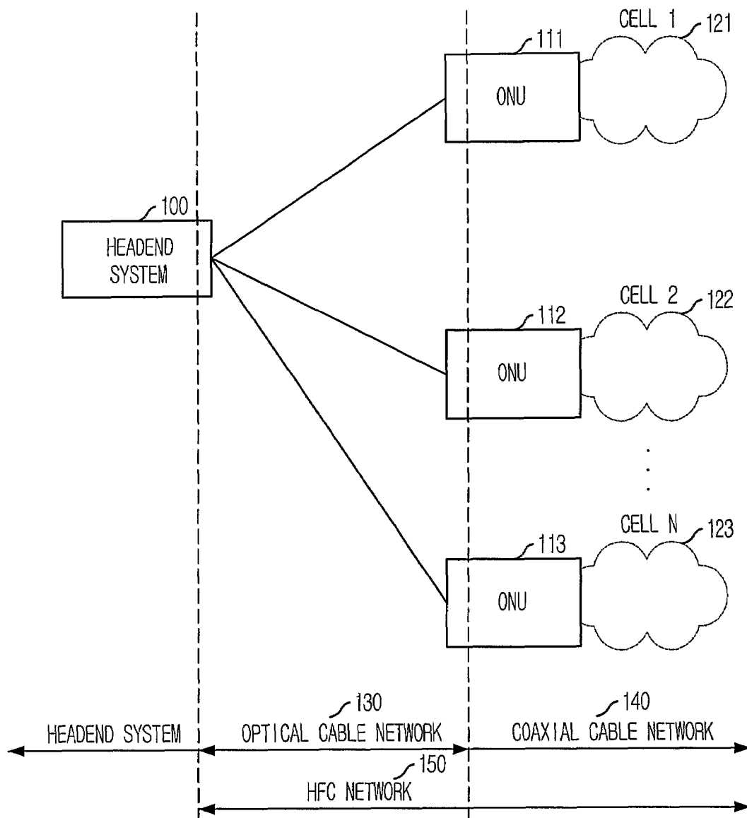
FIG. 1 (PRIOR ART)
