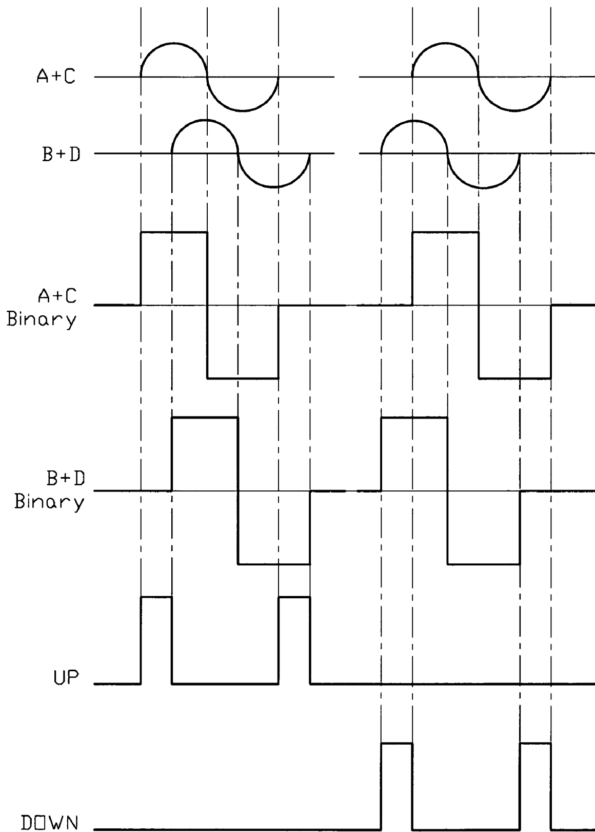
FIG.2(Prior Art)
