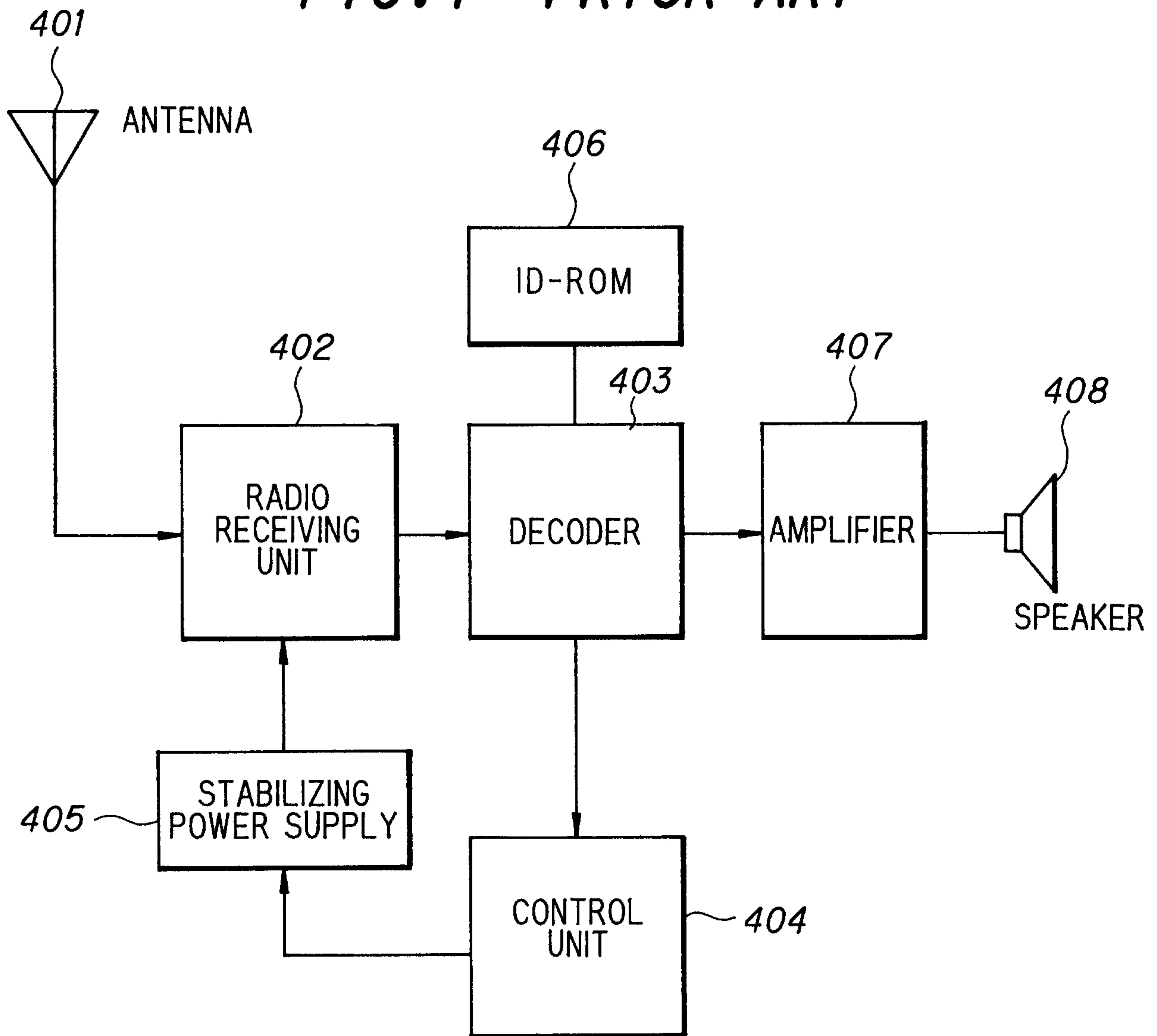
FIG. 1 PRIOR ART
