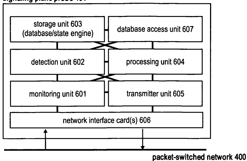
signaling plane probe 401
