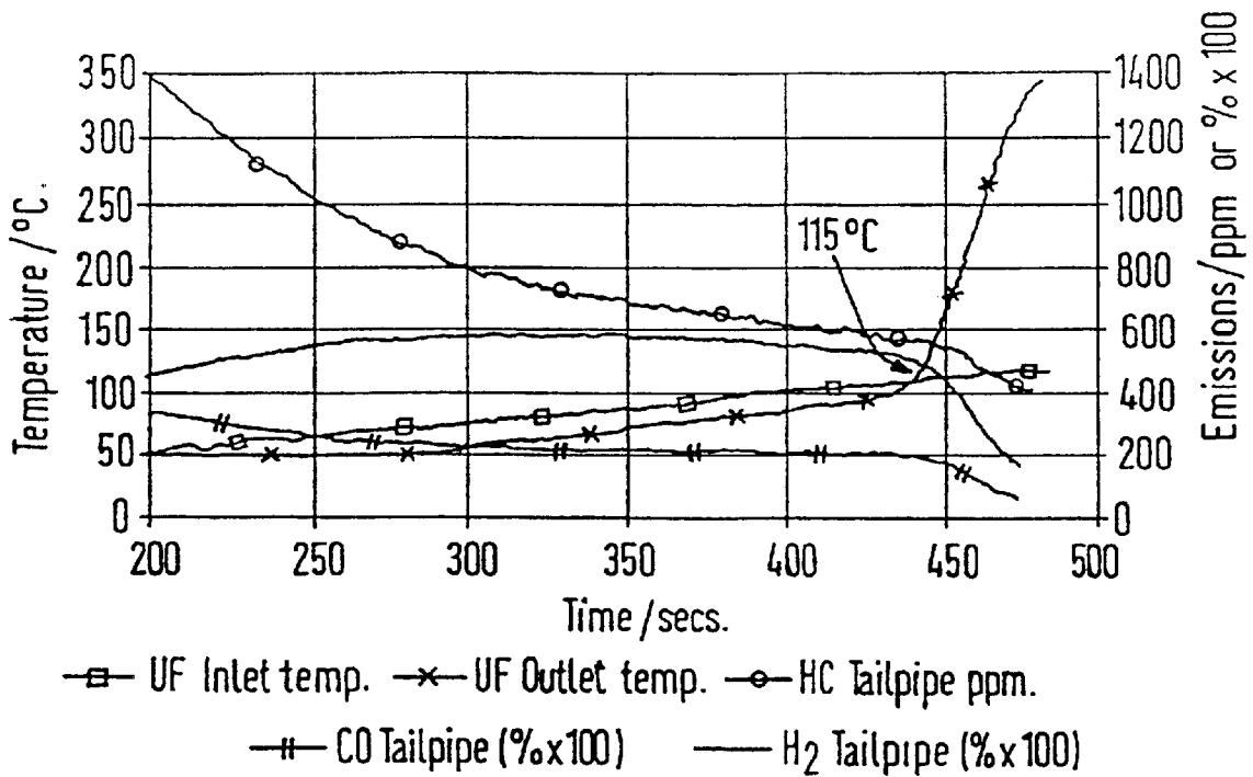
Fig.7. TEST 6 Pre-TWC Trap enhances Light-off further.
