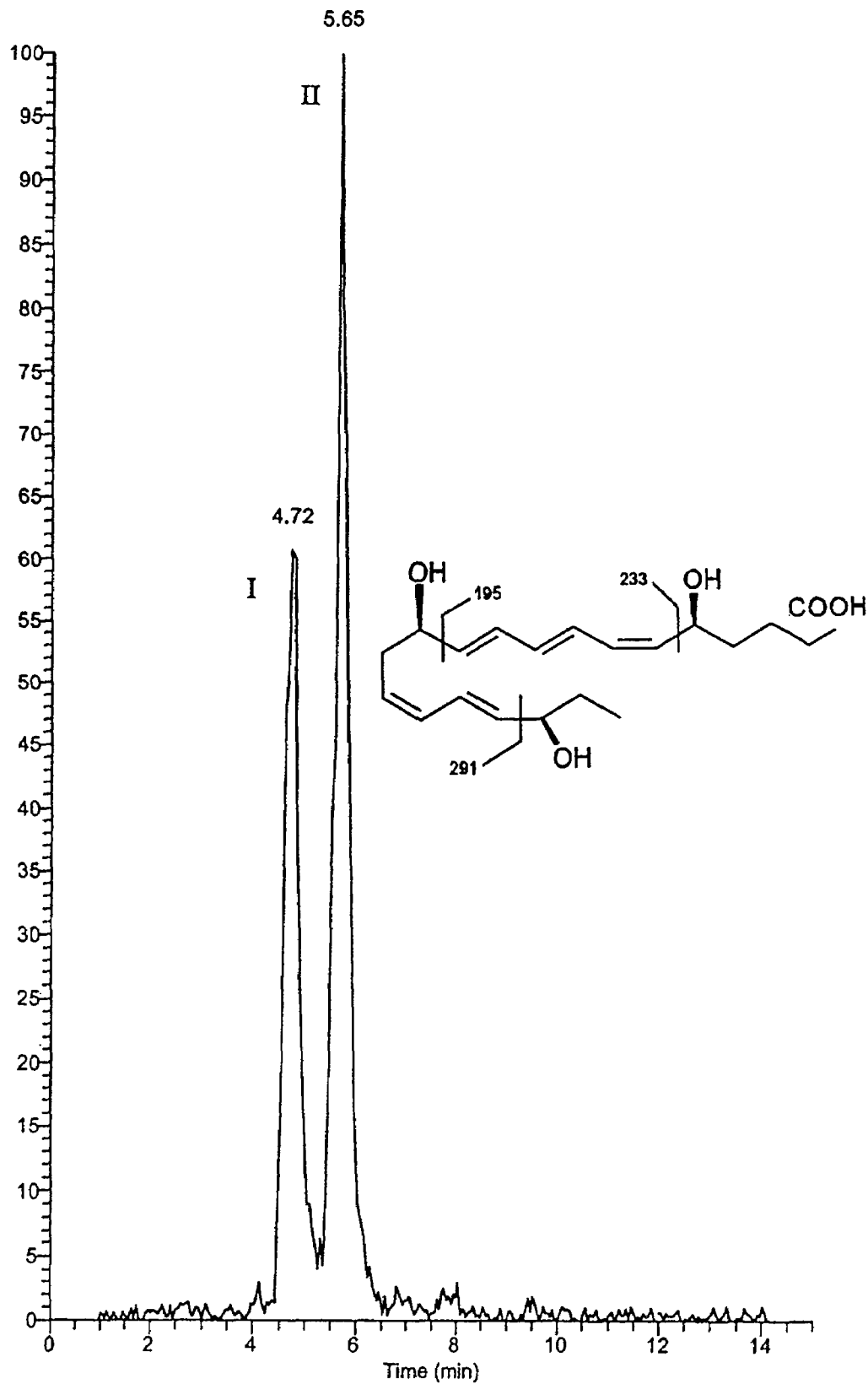
FIG. 5-1 MS 5,12,18-tri-HEPE from B. megaterium
