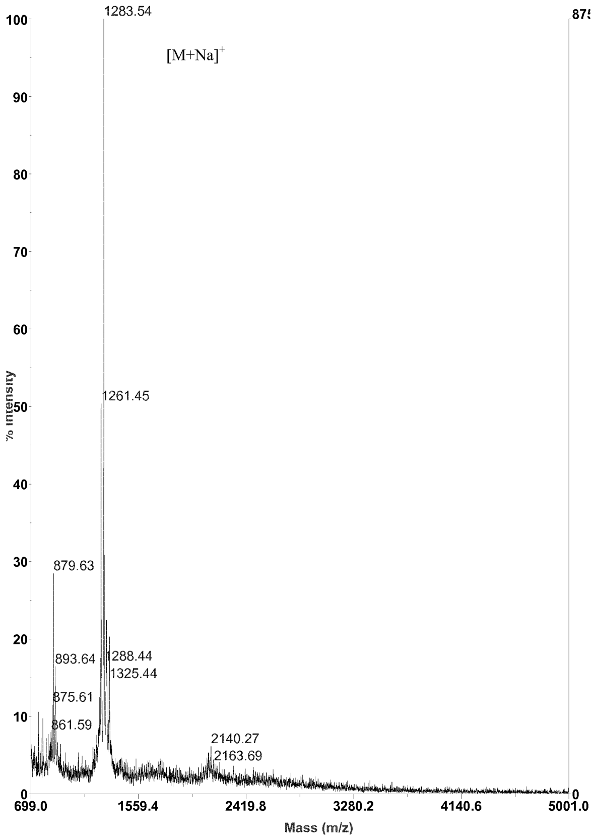
FIG. 19 Voyager Spec #1[BP = 1283.5, 8754]
