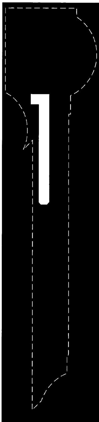
N-Well mask
