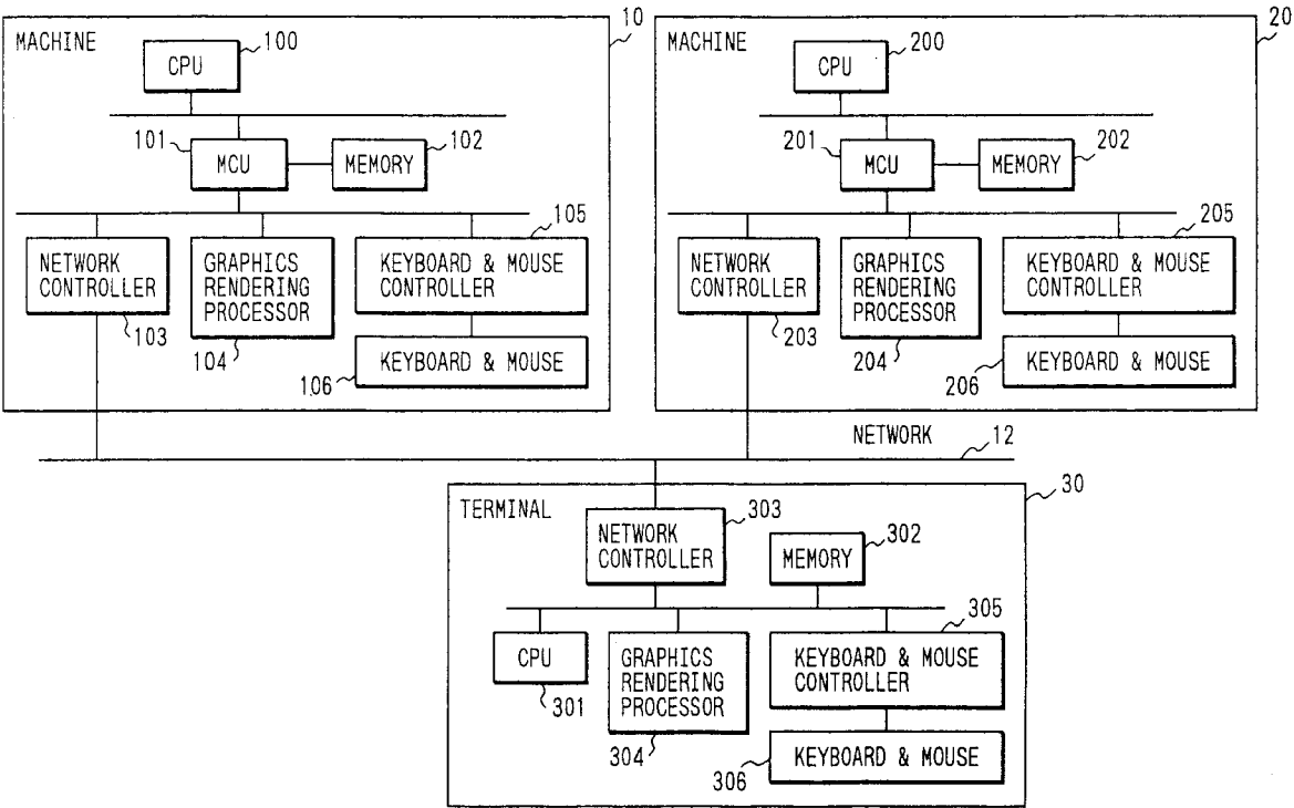
HARDWARE BLOCK DIAGRAM OF GRAPHICS SYSTEM
