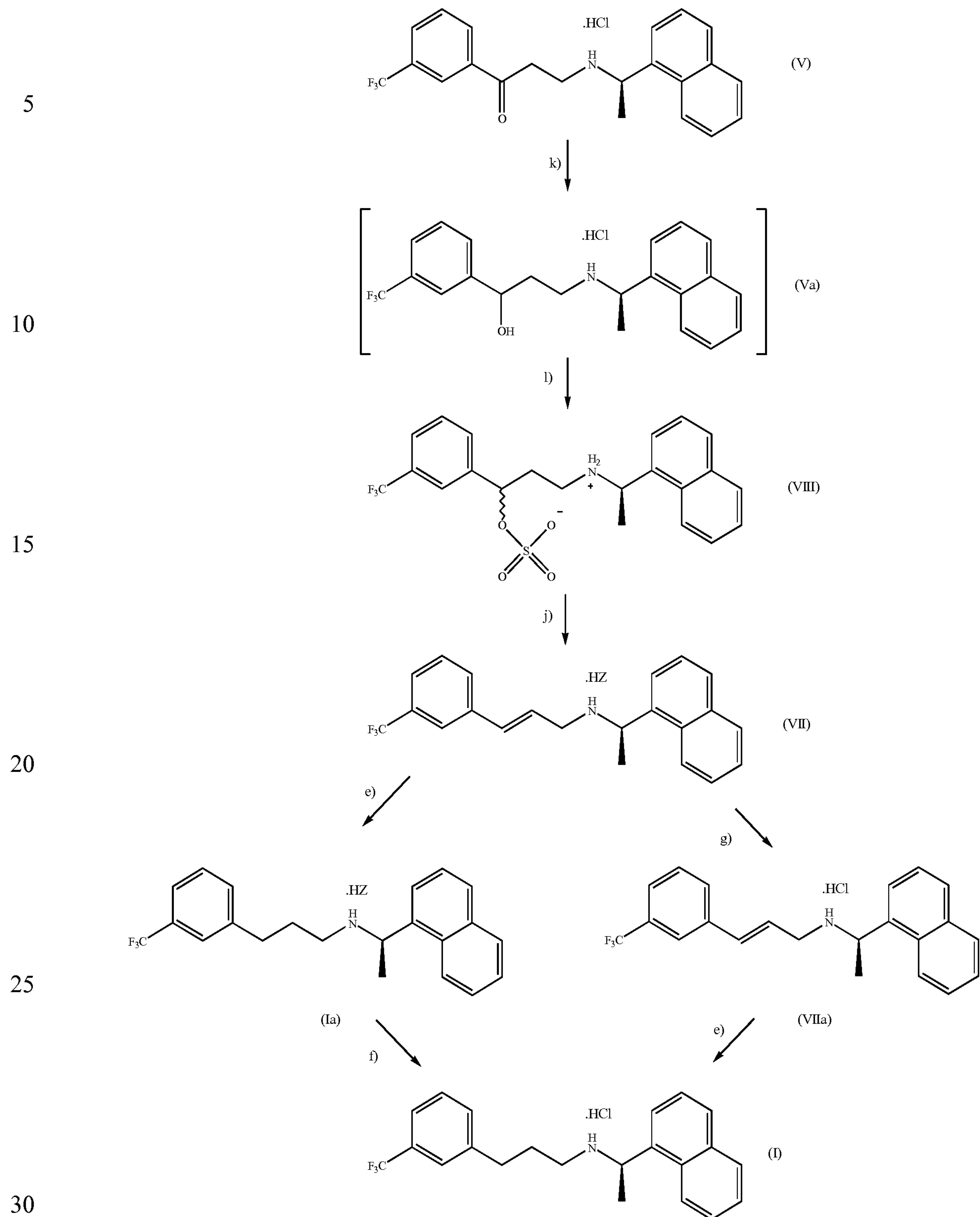
Scheme 2
