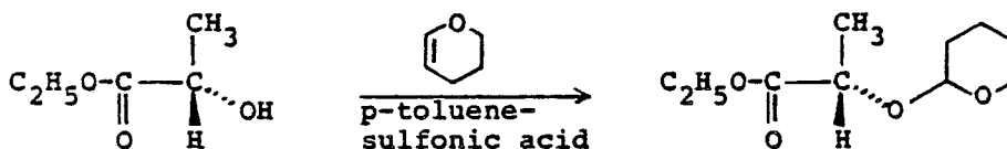
(S)-L-ethyl lactate
