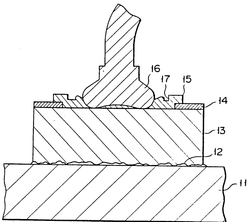
FIG. 2 (PRIOR ART)
