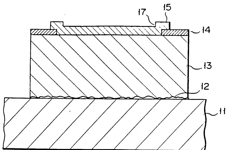
FIG. 1 (PRIOR ART)
