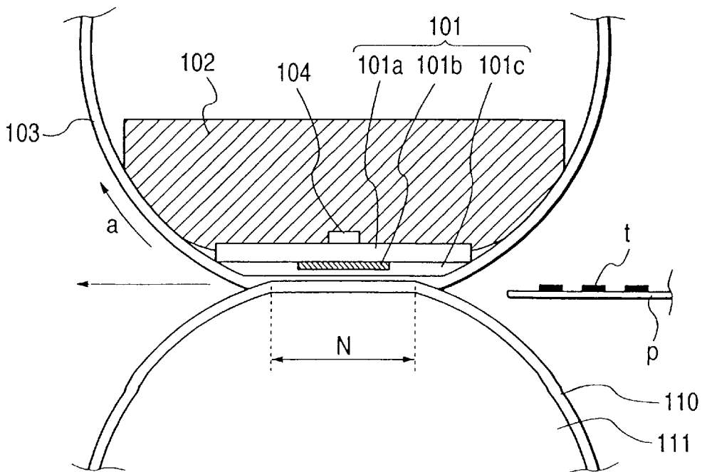
FIG. 13 PRIOR ART
