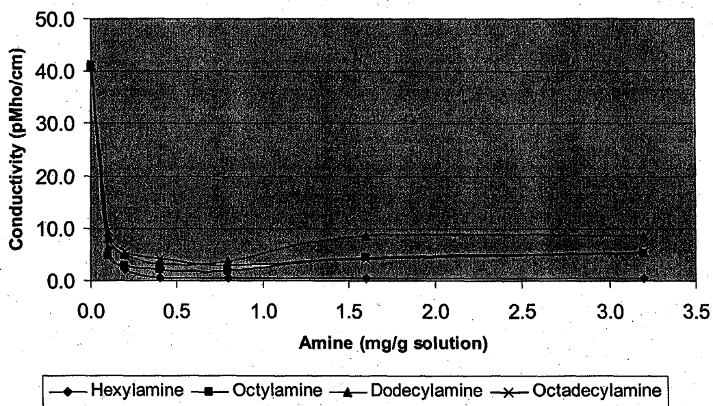
Figure 1, Effect of carbon chain length of amines on toner conductivity.
