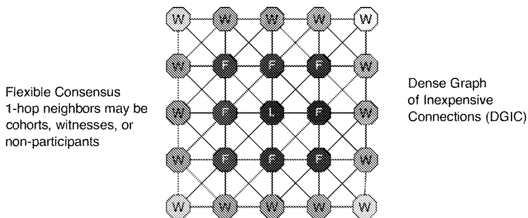
(c) 5 x 5 Consensus Tile
