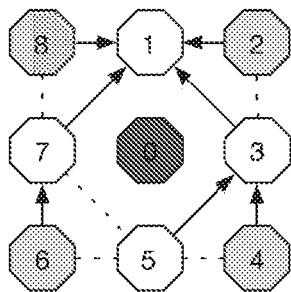
(e) Recovery by election 2 (Paxos)
