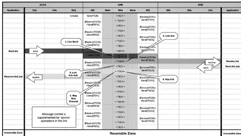
Example 2b: Message Transfer using Link Facilities
