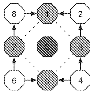
(d) Recovery by election 1 (Paxos)
