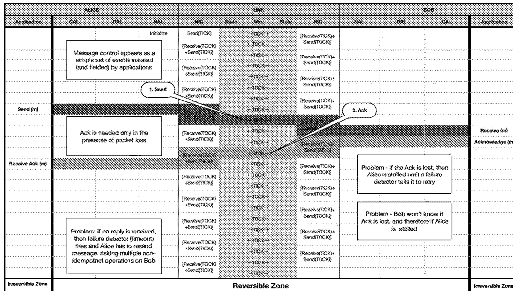
Example 1b: Simple (send/ack) Message Transfer, End to End, not using Link facilities
