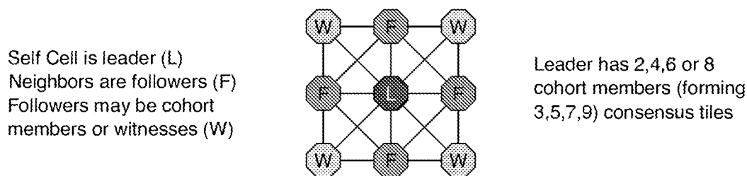
(a) Basic 3 x 3 Consensus Tile
