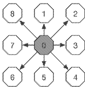
(a) Coordinator initiates Parallel messages
