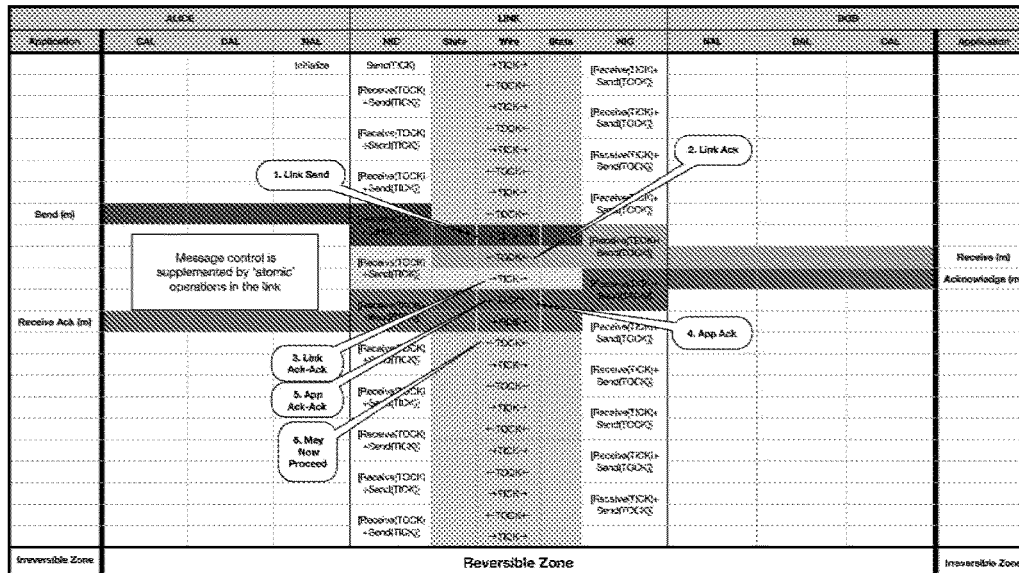
Example 1b: Simple Message Transfer using Link Facilities (Works also for Token Transfer)
