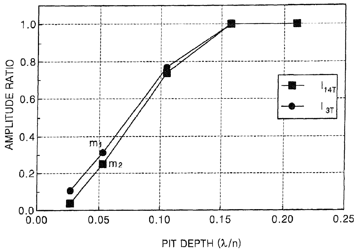
FIG. 3 (PRIOR ART)
