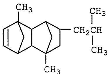
9-Isobutyl-2,7-dimethyltetracyclo- [4,4,0,12.5,17.10]-3-dodecene
