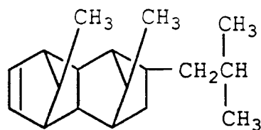
9-Isobutyl-11,12-dimethyltetracyclo- [4,4,0,12.5,17.10]-3-dodecene
