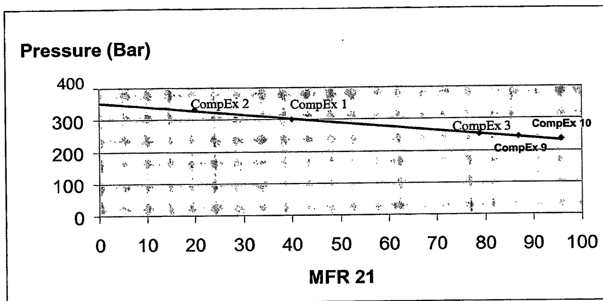
Fig.1: Extruder pressure as a function of MFR 21
