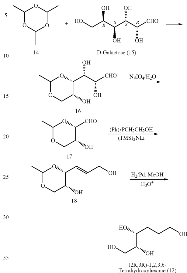
Scheme 2: Synthetic procedures for preparation of (2R,3R)-1,2,3,6-tetrahydroxyhexane (12)
