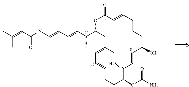
Scheme 12. Retrosynthetic analysis of palmerolide A (1)
