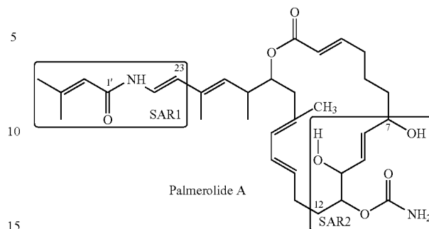
Scheme 7: Natural product diversity based on structure-activity profile
