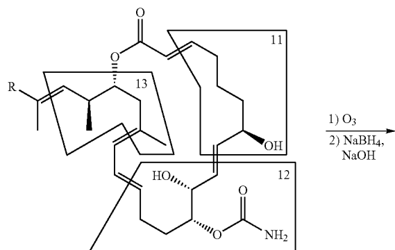
Scheme 1: Degradation studies (ozonolysis of parmerolides A (1), D (8) and E (9)).
