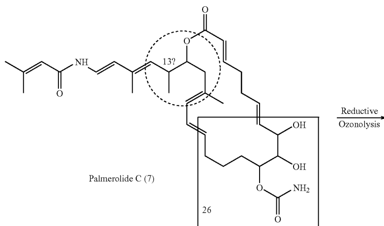
Scheme 5. Ozonolysis of palmerolide C (7).
