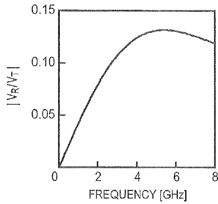
FIG. 1 PRIOR ART
