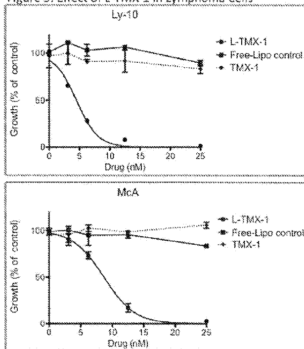
Figure 9: Effect of L-TMX-1 in Lymphoma Cells
