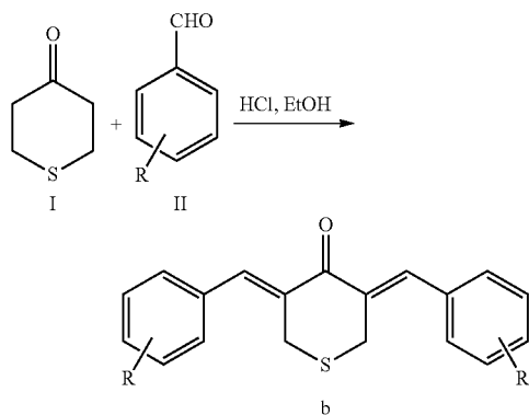
Scheme 1. General procedure for the synthesis ofsynthetetrahydro-3,5-bis[phenylmethylene]-4H-thiopyran-4-one derivatives
