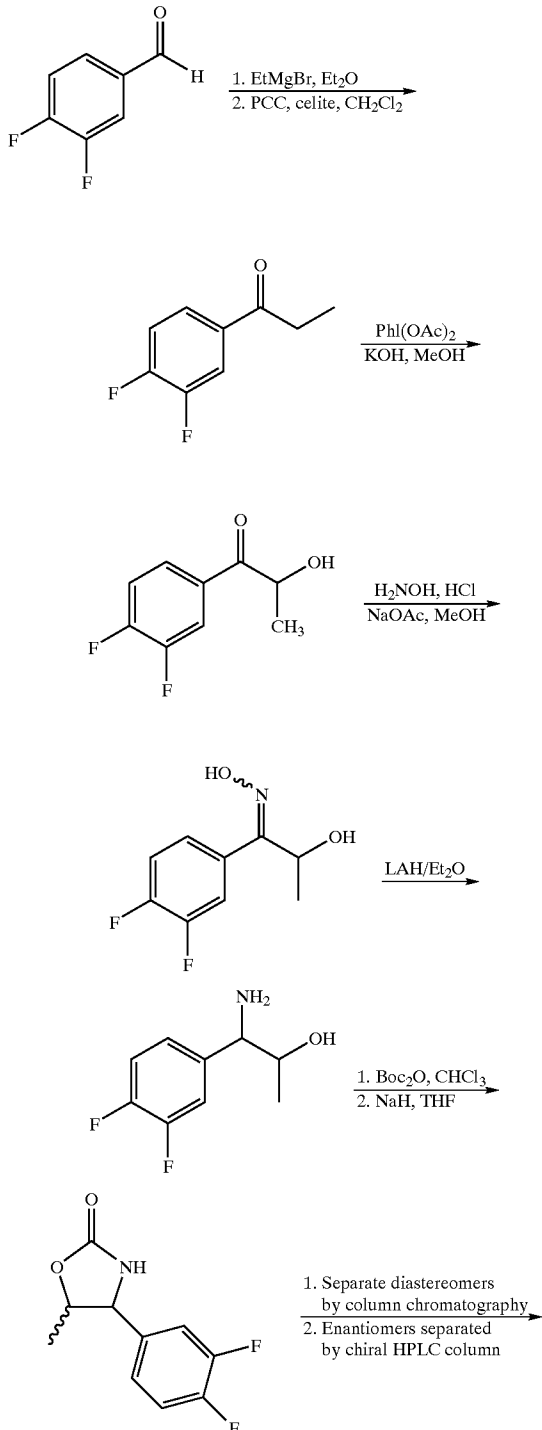
Scheme 3
