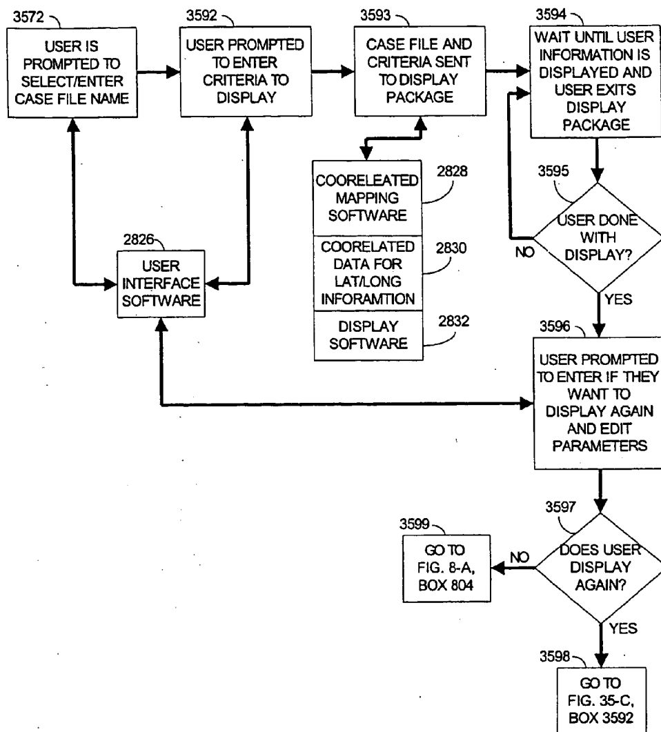
PRIMARY ANALYTIC SOFTWARE (CONTINUED)
