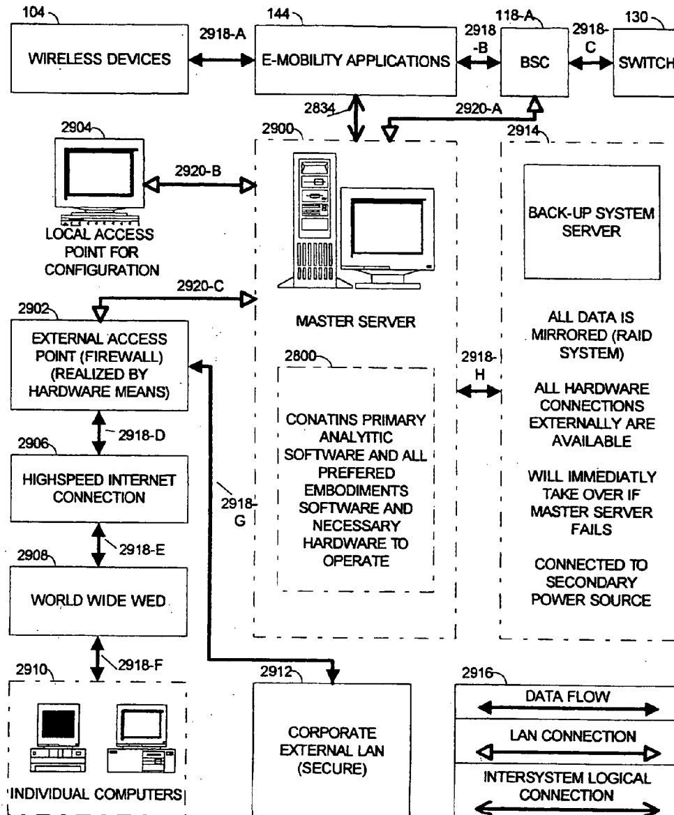
PHYSICAL REALIZATION OF PREFERRED EMBODIMENTS
