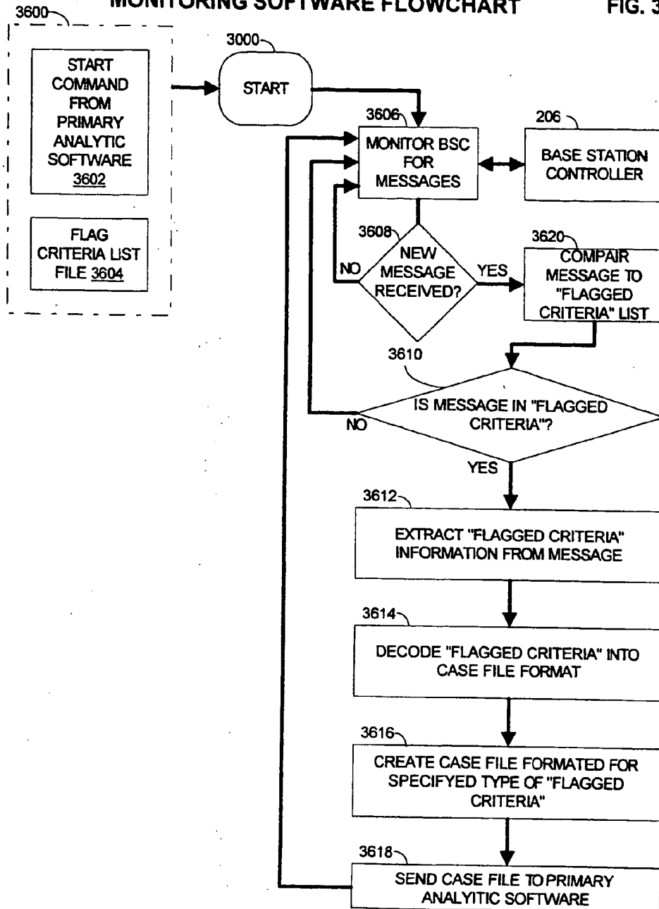
MONITORING SOFTWARE FLOWCHART
