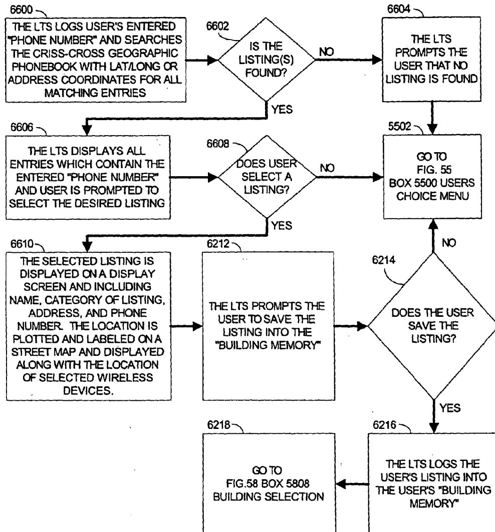
"PHONE NUMBER" ADDED TO "BUILDING MEMORY"
