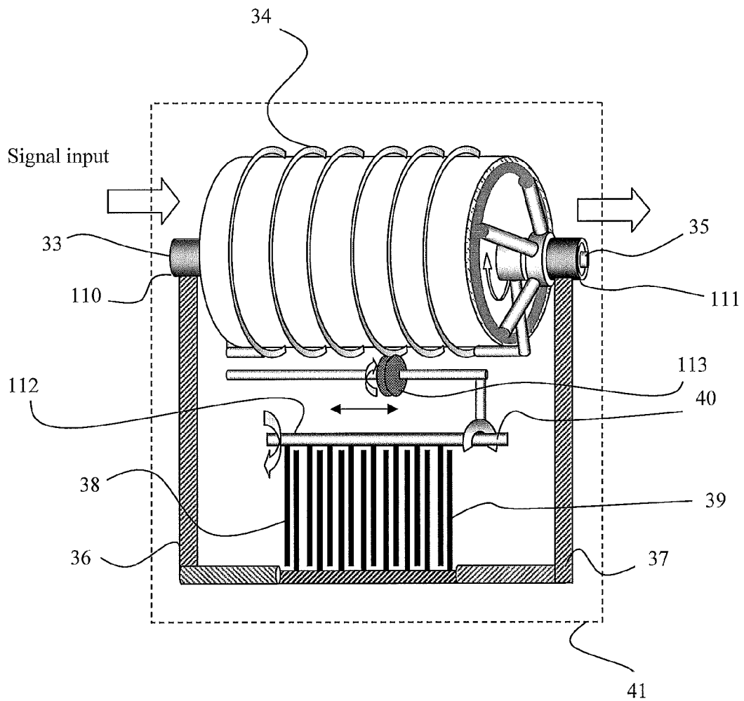
FIGURE 11: Low frequency impedance tuner
