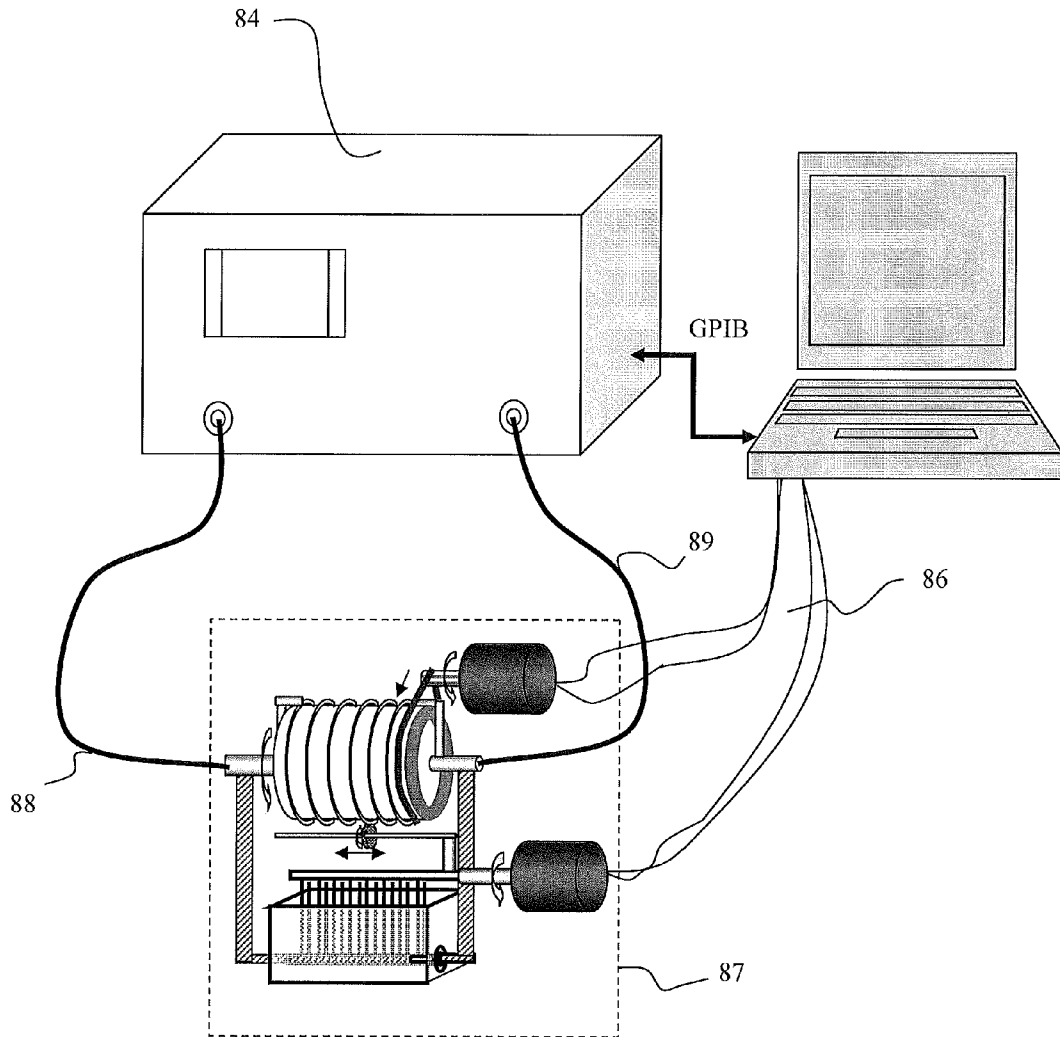
FIGURE 25: Tuner calibration setup
