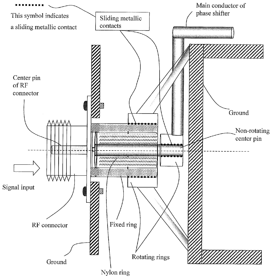
FIGURE 10: Coaxial adapter transition to rotating phase shifter.
