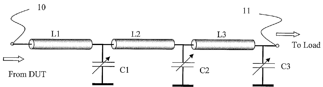
FIGURE 5: Prior art, triple Line-Capacitor impedance tuner
