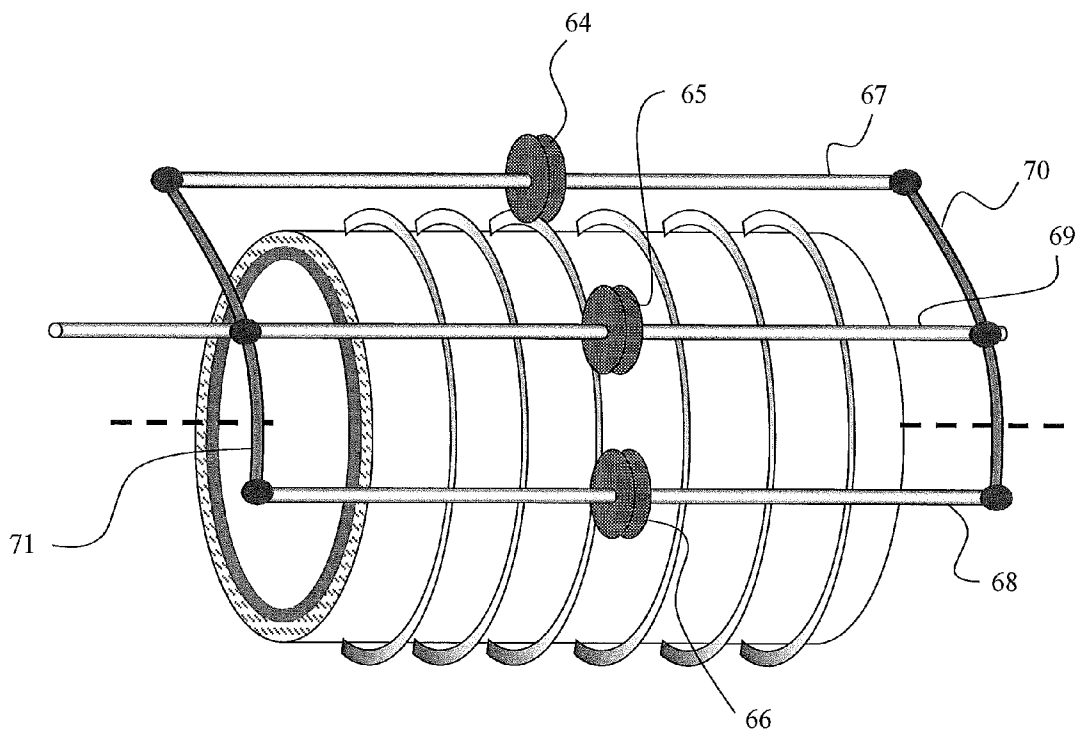
FIGURE 19: Linear, high power, phase shifter.
