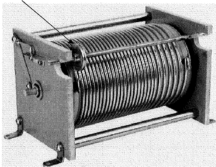
FIGURE 14 b): Prior art, variable rotating inductor
