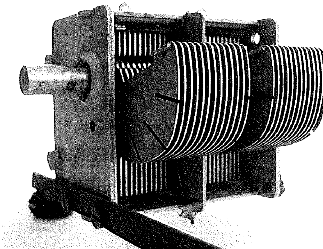
FIGURE 14 a): Prior art, variable rotary capacitor
