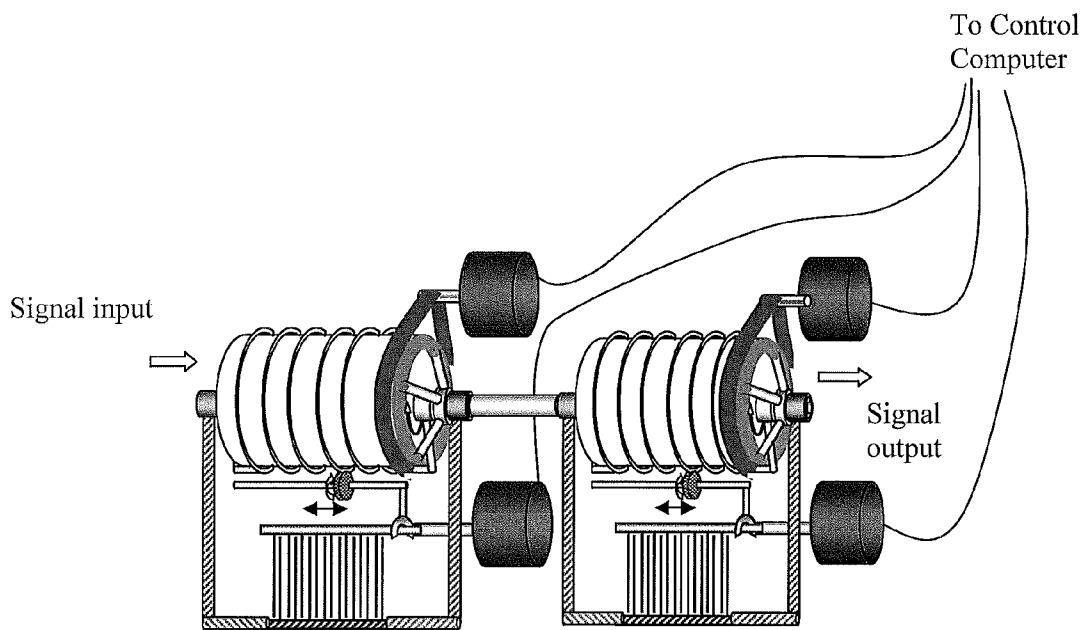
FIGURE 22: Two stage pre-matching or two-frequency harmonic tuner
