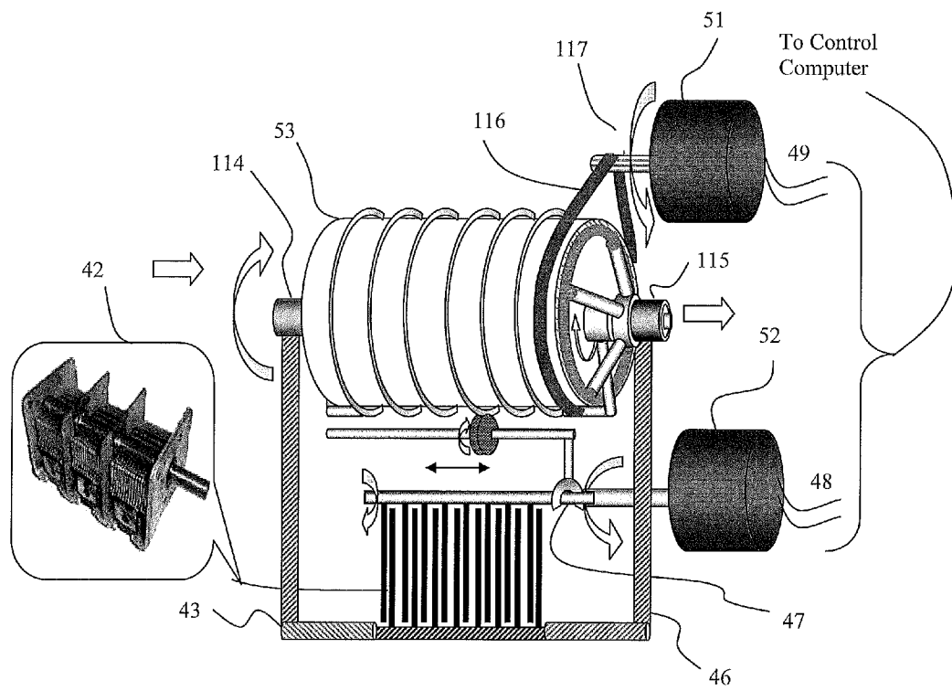
FIGURE 12: Automated low frequency impedance tuner
