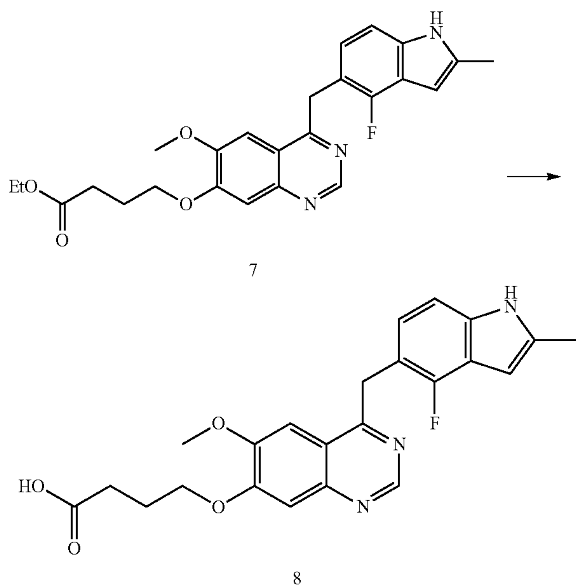
Scheme 2C
