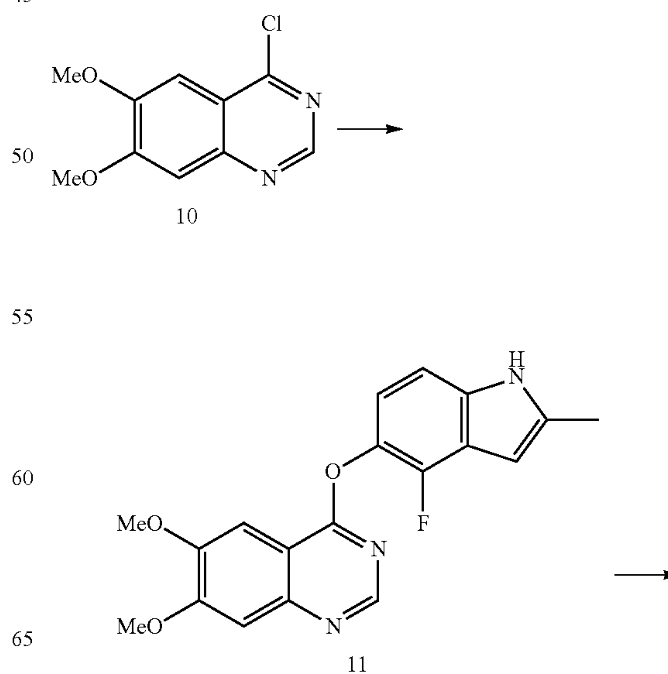
Scheme 3
