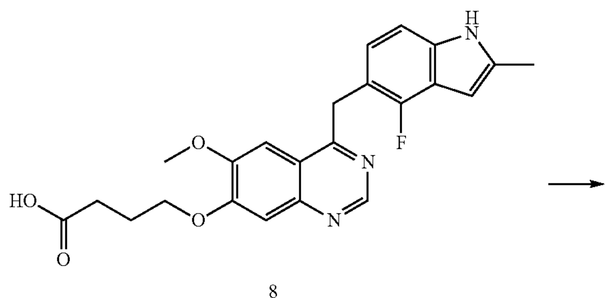
Scheme 2D
