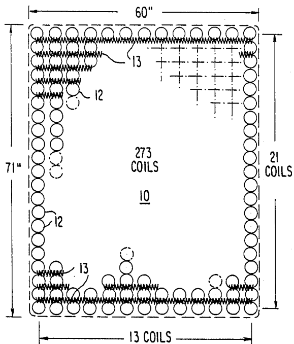
FIG. 1 PRIOR ART
