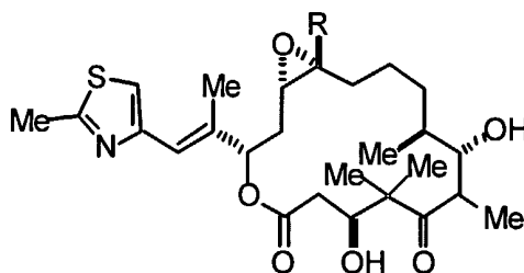
Epothilone A R=H
