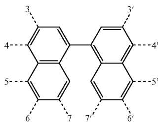
1, 1'-binaphthylene
