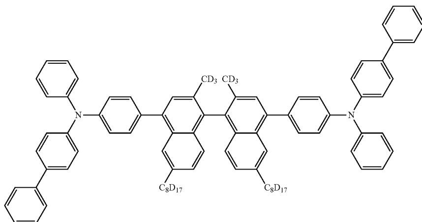
Compound A:
