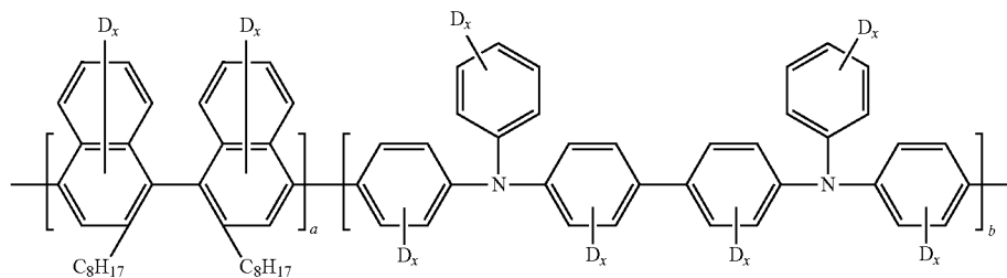
Compound I:
