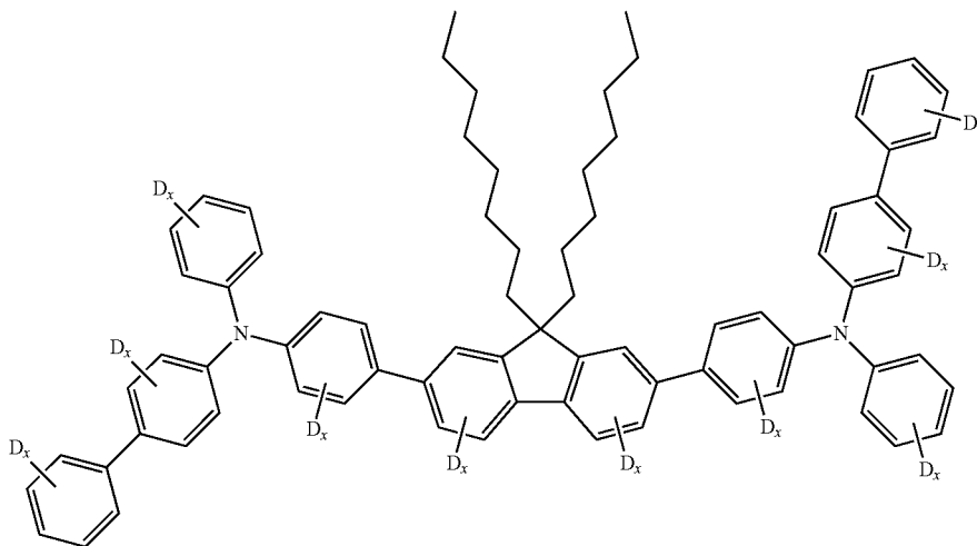
Compound P:
