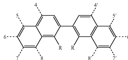
2, 2'-binaphthylene
