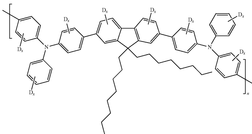
Compound P:
