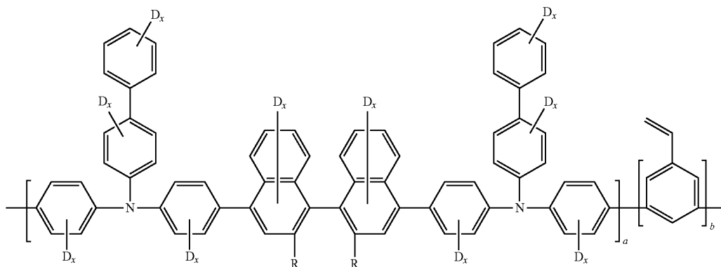
Compound K:
