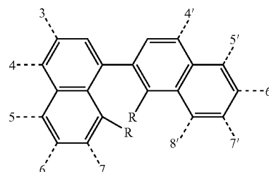
1, 2'-binaphthylene
