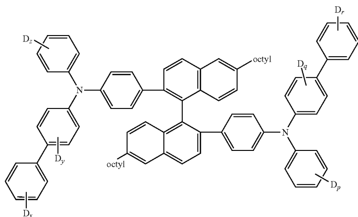
Compound B:
