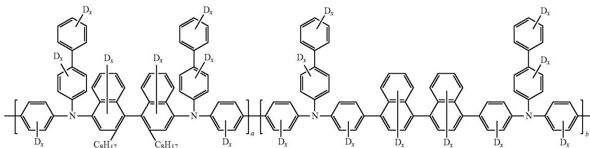
Compound J:
