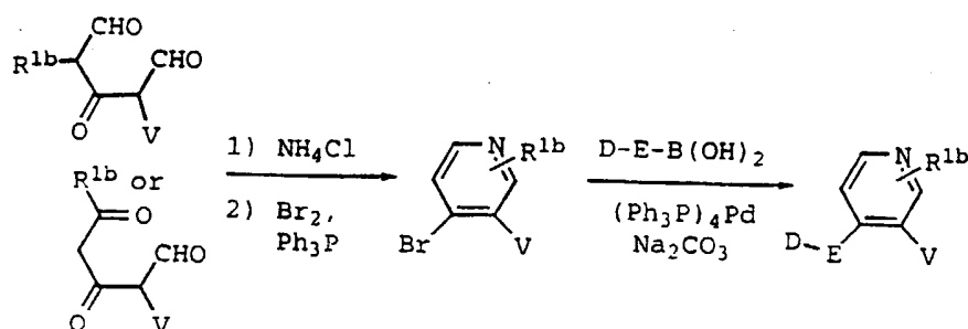
Scheme 44
