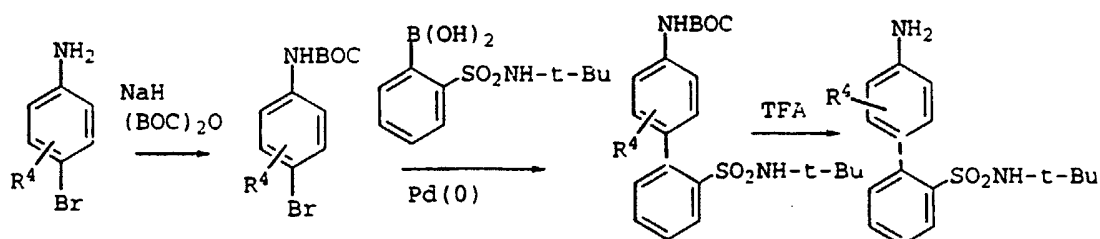
Scheme 58
