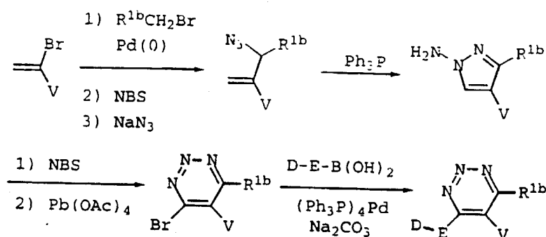
Scheme 52
