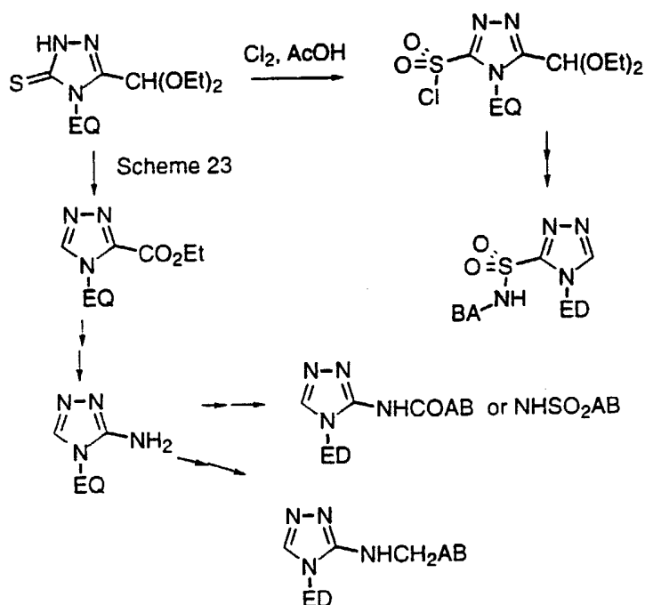
SCHEME 34
