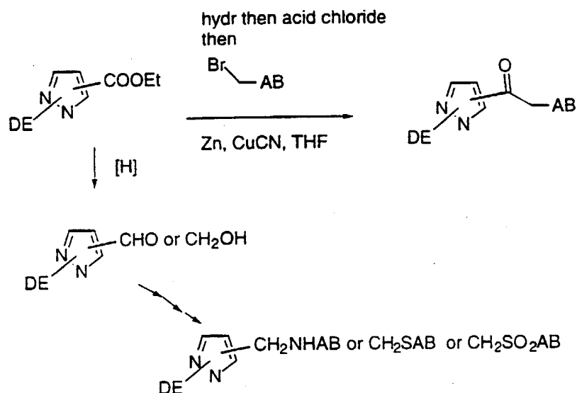
SCHEME 23
