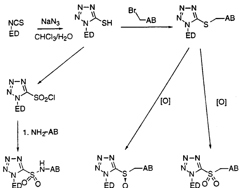
SCHEME 16
