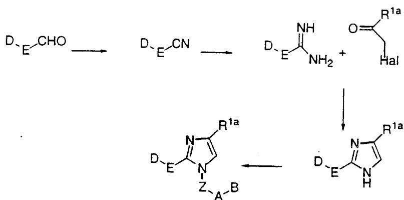
SCHEME 19
