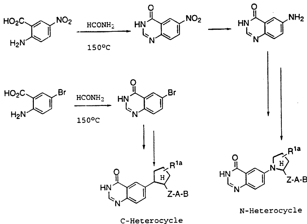
SCHEME 11
