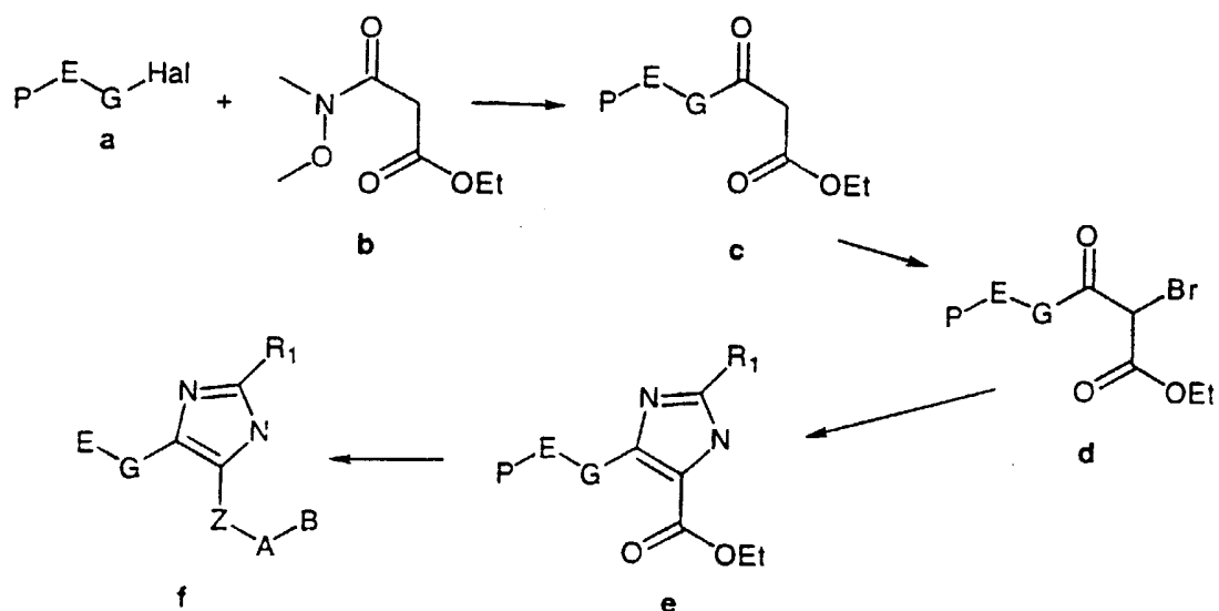
Scheme 18b
