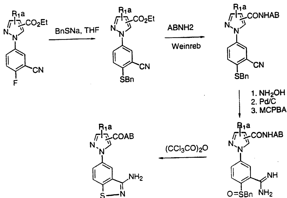
SCHEME 13
