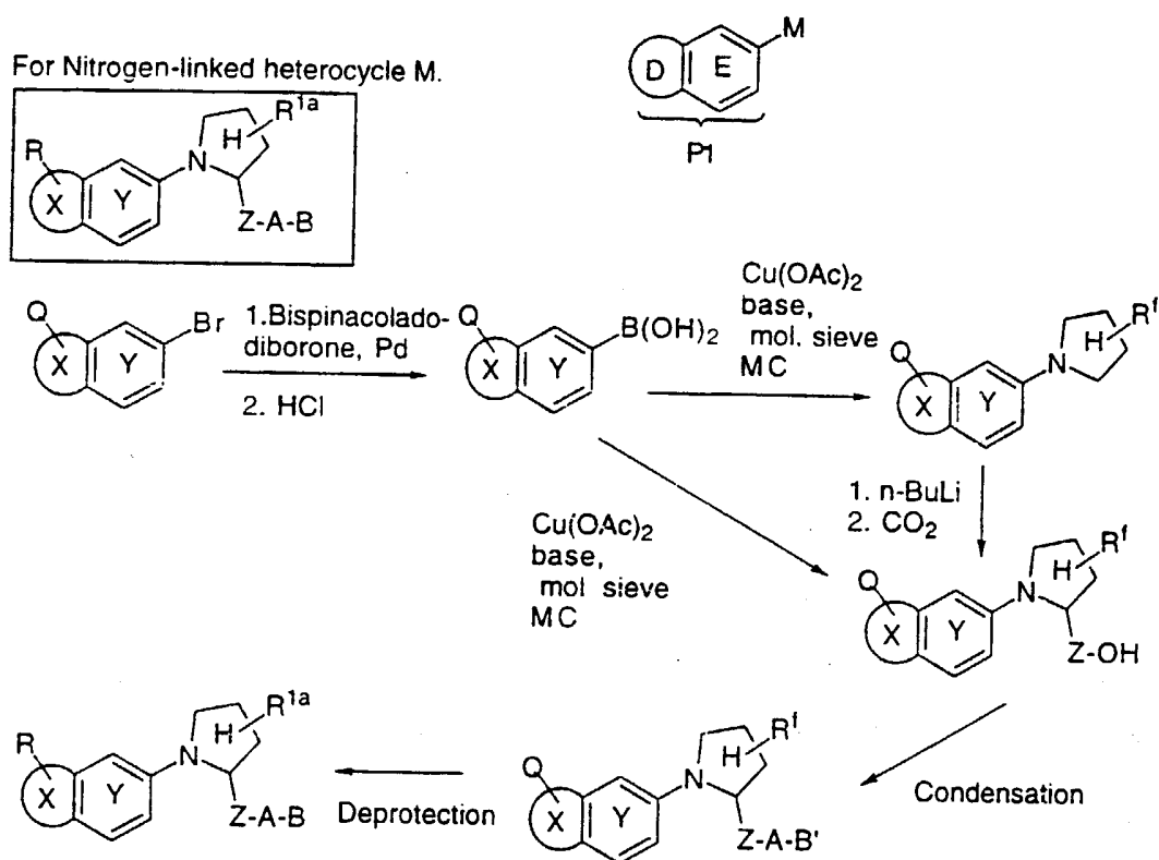
SCHEME 59
