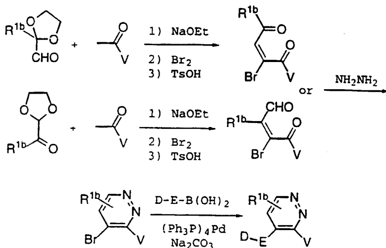
Scheme 48
