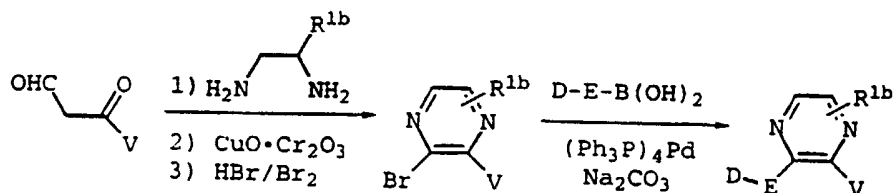
Scheme 51
