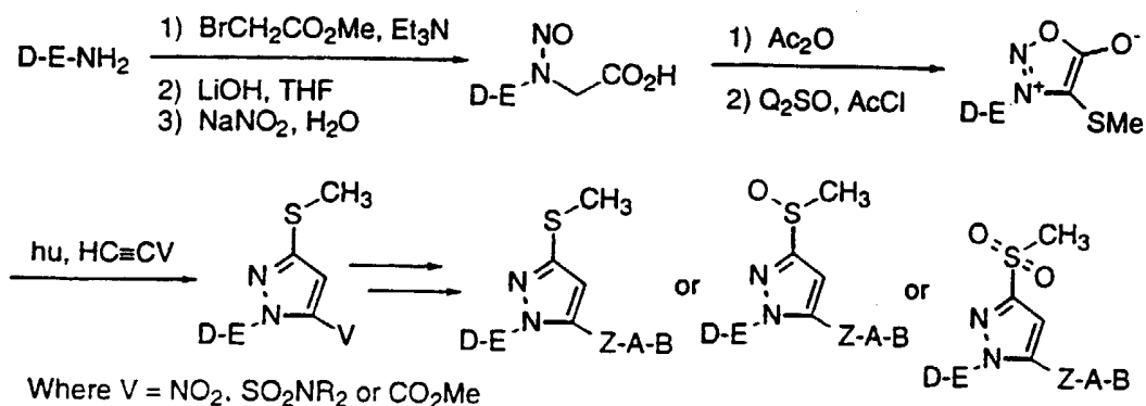
SCHEME 35
