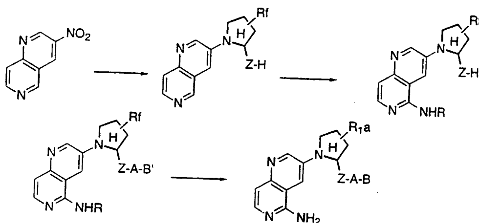
SCHEME 2b
