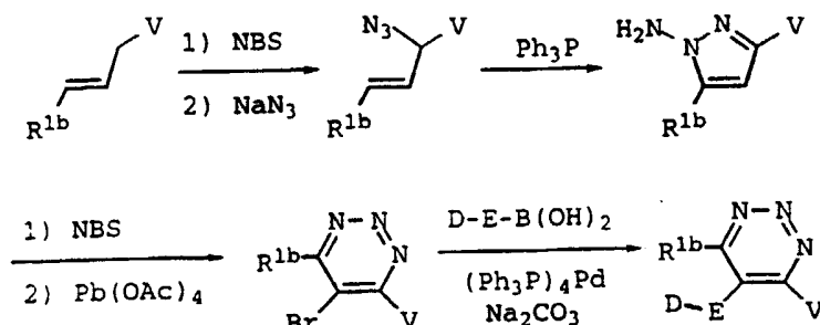
Scheme 53
