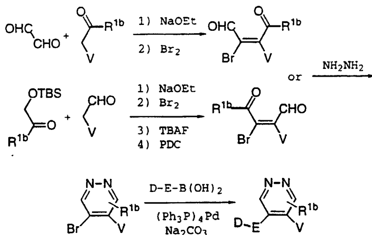
Scheme 47
