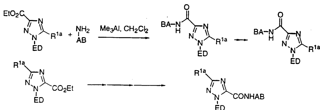
SCHEME 29
