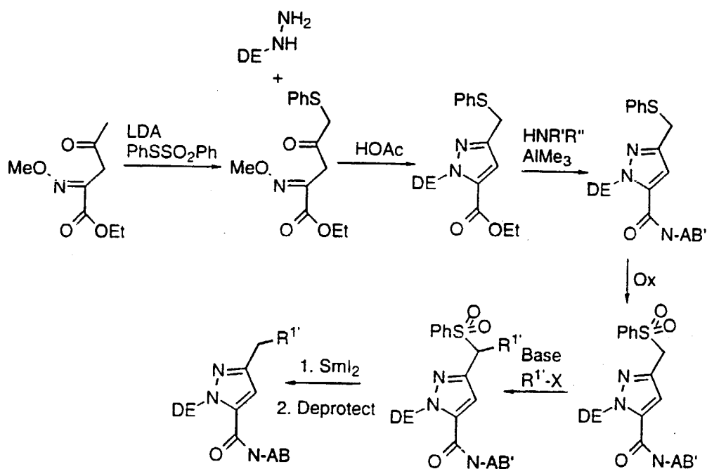
SCHEME 38
