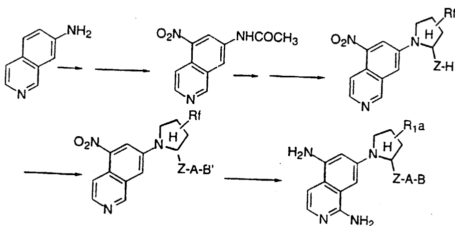
SCHEME 2c
