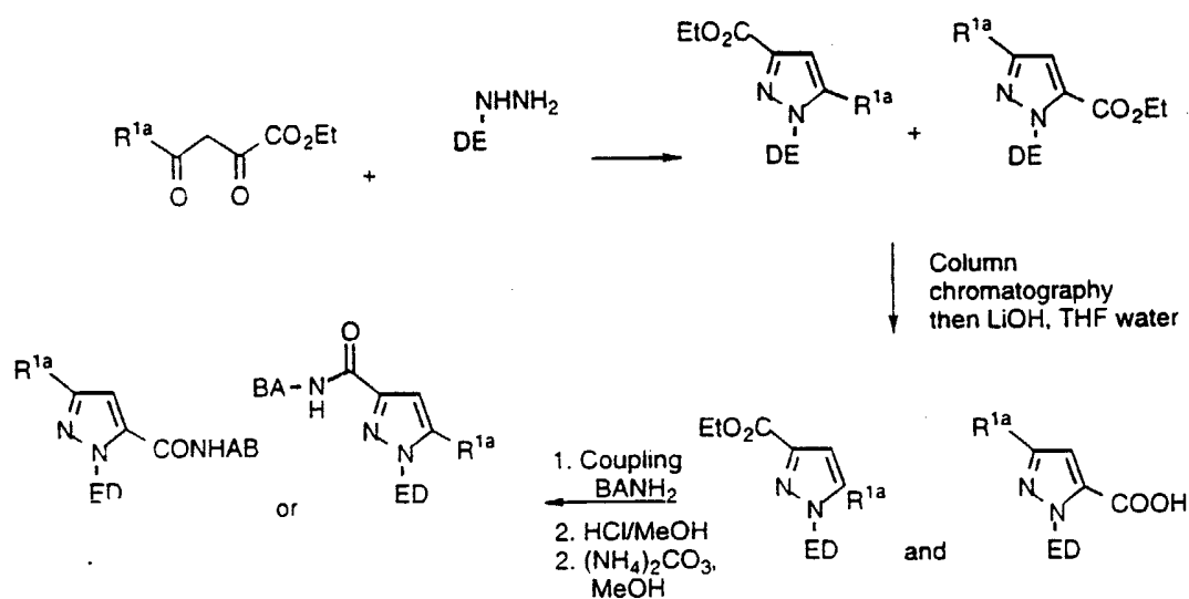
SCHEME 20
