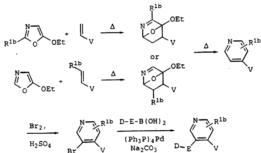
Scheme 43
