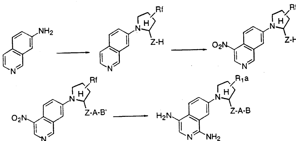
SCHEME 2d
