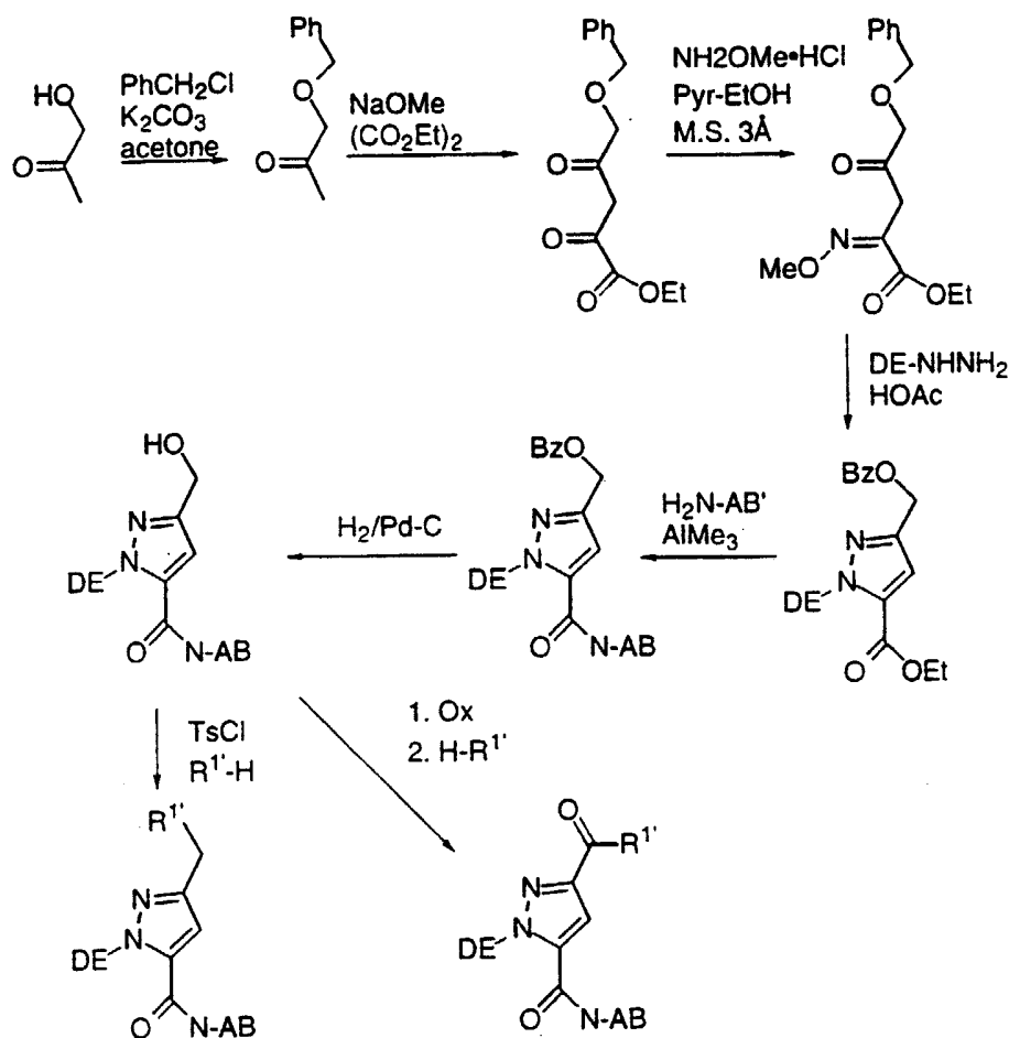
SCHEME 39
