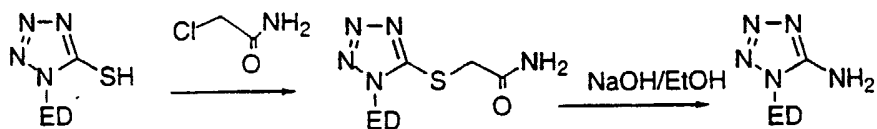
SCHEME 17
