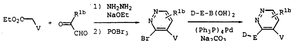
Scheme 46
