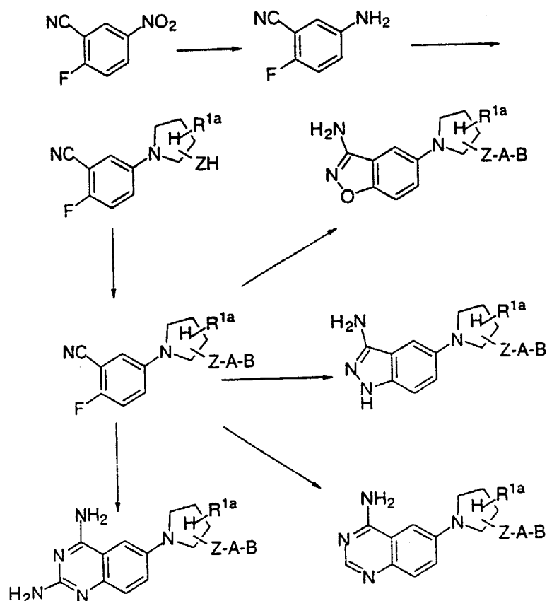
SCHEME 7
