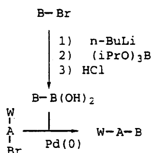
Scheme 57
