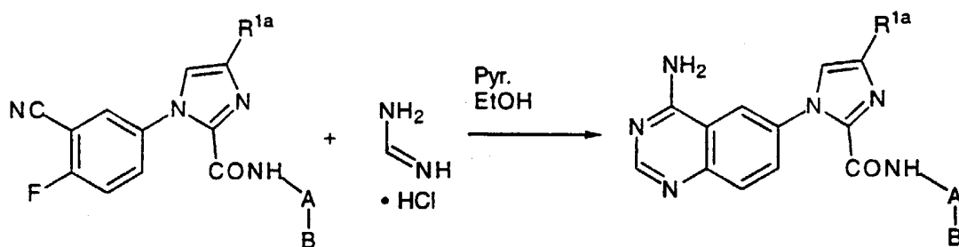
SCHEME 61
