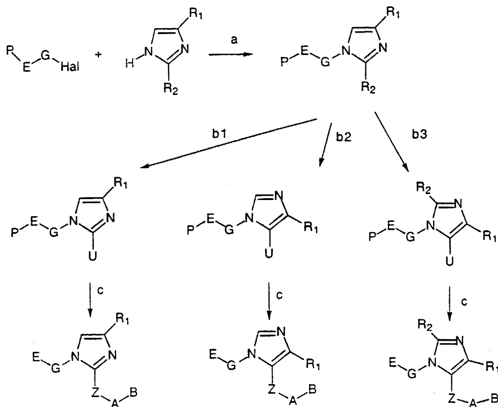
SCHEME 18a
