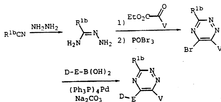
Scheme 54
