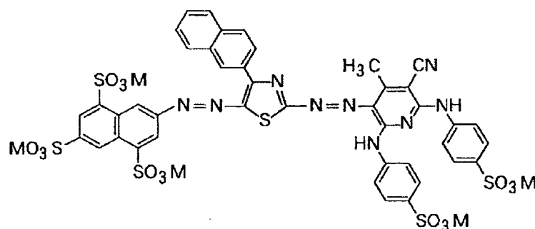
Chem. 1
