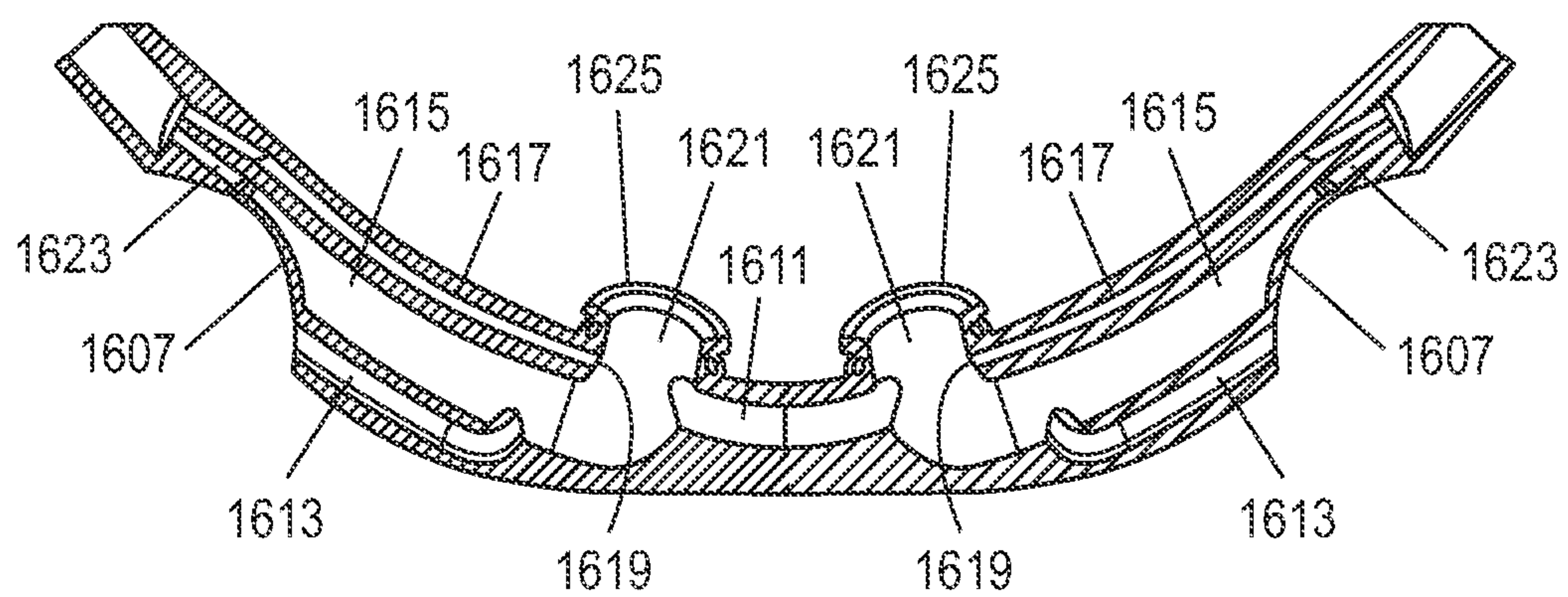
FIG. 18 SECTION E-E
