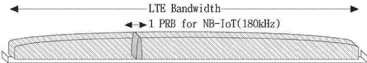
In-band Mode
