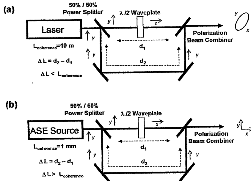
Figure 6 - Schematic of the optical elements of a depolarizer and a pictorial illustration of polarization state for (a) long and (b) short coherence sources.
