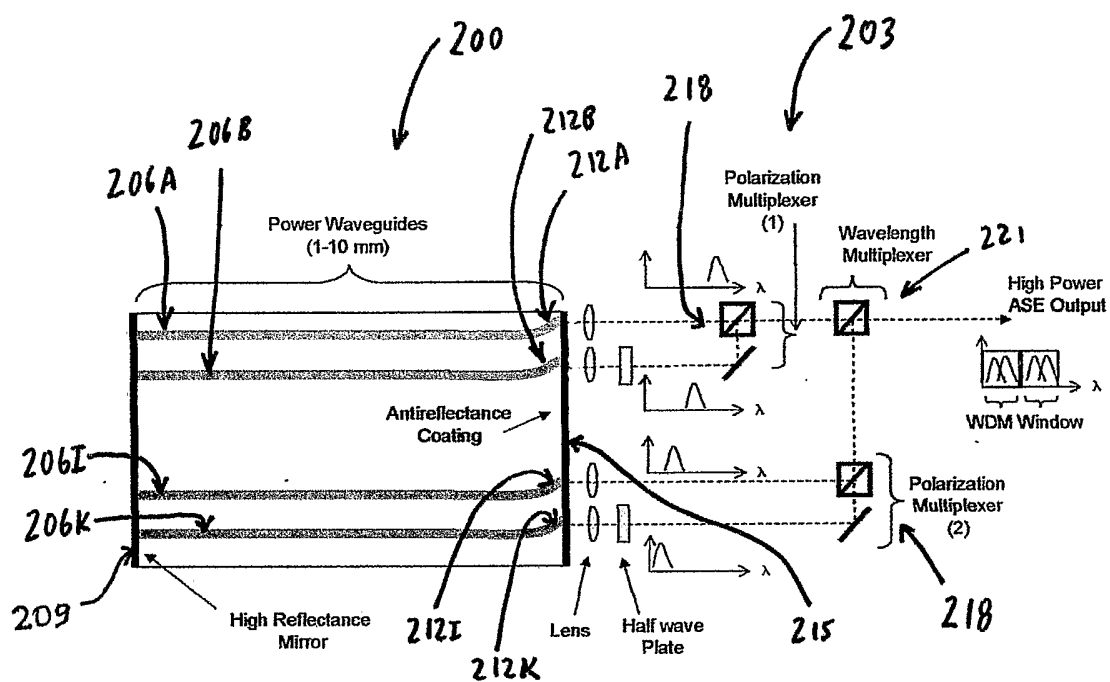
Figure 11- A schematic of the semiconductor die and optical train for preferred embodiment #2
