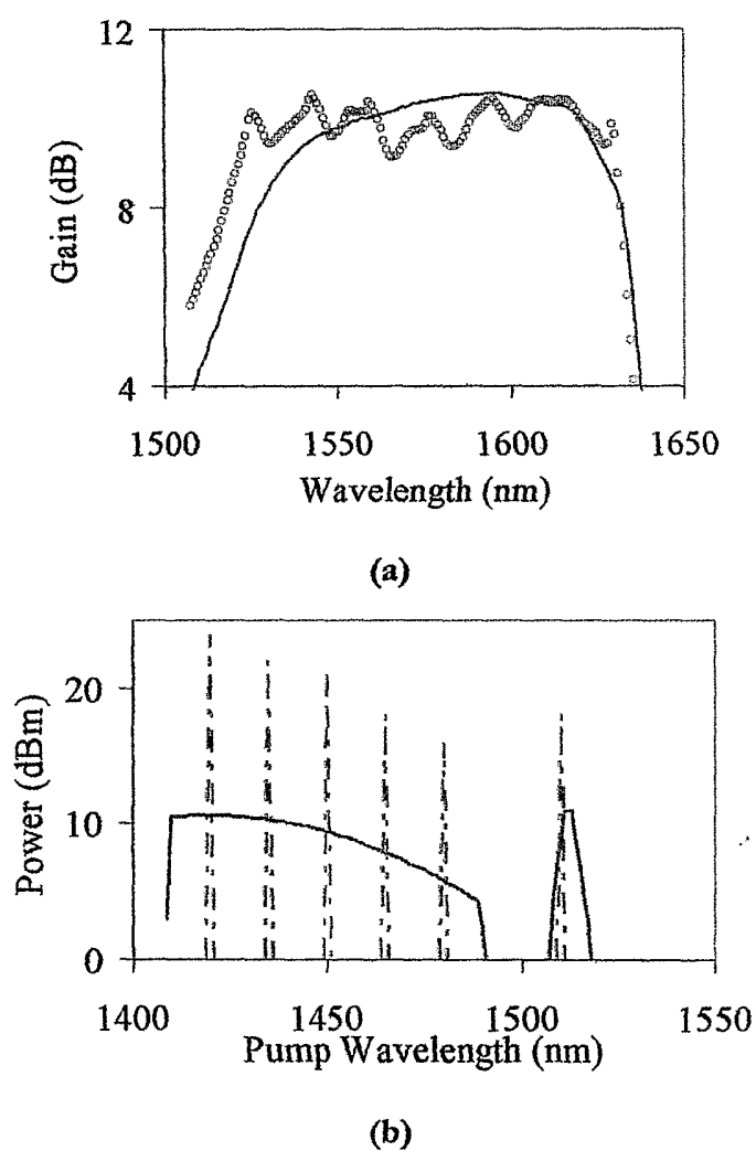
Figure 5 - Simulated Raman gain shape (a) achieved using 6 discrete pump wavelengths (open dots) and that with 2 broadband sources (solid curve). The pump wavelength and power distribution are shown in the lower plot (b).
