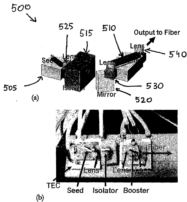
Figure 14 - The Use of a Discrete Seed and Booster to Generate High Power ASE. (a) shows the schematic of the experimental setup and (b) presents a photograph of the actual microoptical bench setup.
