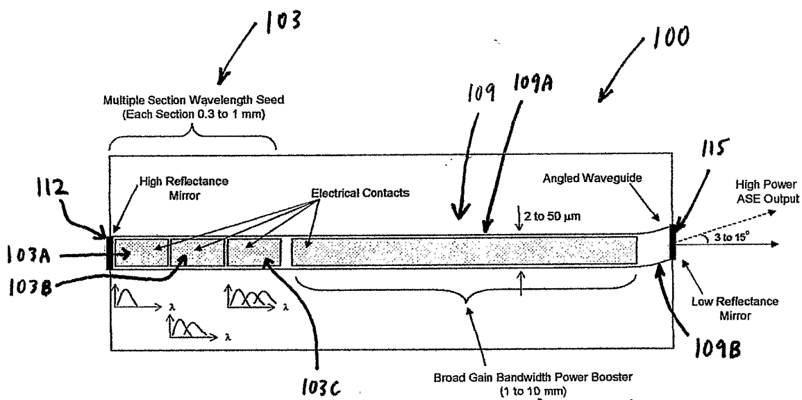
Figure 10 - Shows a schematic of the semiconductor chip for preferred embodiment #1. The chip consists of a serial connection of a wavelength seed section and a power booster or power amplification section.
