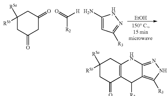
Scheme 1a. Synthesis Protocol A
