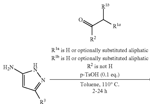
Scheme 1c. Synthesis Protocols C to F.
