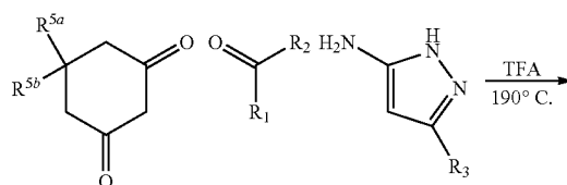
Scheme 1b. Synthesis Protocol B
