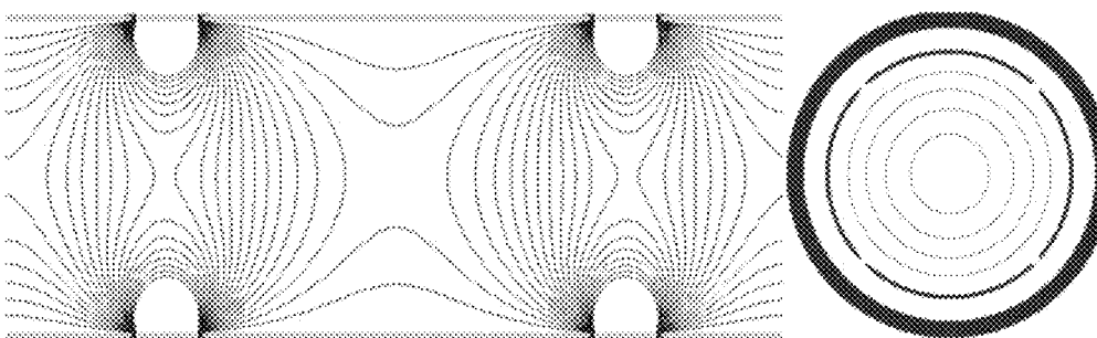
Standard cylindrical ICR cell:
